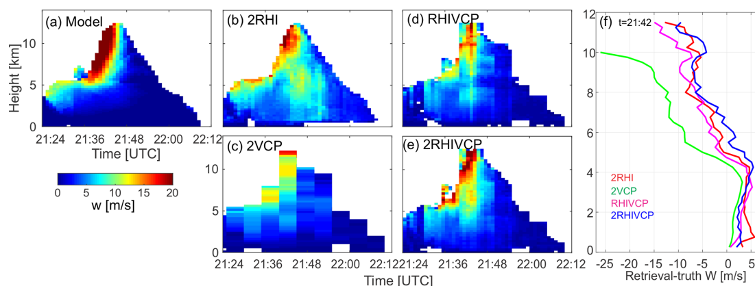
Figure 8. Height–time cross sections of the updraft velocity averaged over the area with reflectivity > 40 dBZ from (a) the model (truth) and (b–e) the simulated retrievals, as well as the (f) errors of the simulated multi-Doppler vertical velocity retrievals (retrieval–truth) at 21:42 UTC, when the maximum updraft was produced by the cell.
