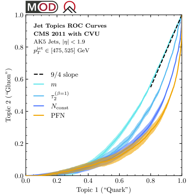
FIG. 15. Extracted ROC curves from the CMS 2011 Open Data. We consider four discriminants that span the range of quark/gluon tagging performance: jet mass, 2-subjettiness, constituent multiplicity, and PFN classification. The fact that the ROC curves slopes are close to 0 and \infty at the end-points imply that the jet topics are mutually irreducible, as desired. For jet mass, the dashed black slope corresponds to the leading-logarithmic prediction in Eq. (59). The error band corresponds to statistical uncertainties propagated through Eqs. (56) and (57).
