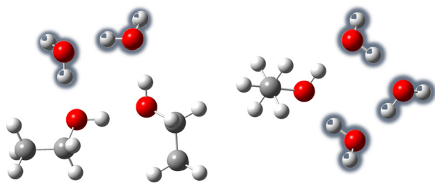
Fig. 4 Comparison of isotopically labeled clusters and actual hydrogen bond position for the wttw conformer of (\text{D}_2\text{O})_2(\text{CH}_3\text{CH}_2\text{OH})_2 and the gwww conformer of (\text{D}_2\text{O})_3(\text{CH}_3\text{CH}_2\text{OH}) .
