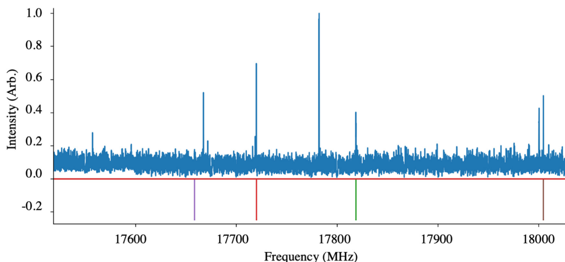
Fig. 1 Section of experimental spectrum with lines fit for various EtOH–water tetramer species. Pictured are lines fit to the (\text{H}_2\text{O})_2(\text{C}_2\text{H}_5\text{OH})_2 wg1tw (green)/wttw (red) and (\text{H}_2\text{O})(\text{C}_2\text{H}_5\text{OH})_3 wg1g2t (purple)/wttt (brown) tetramers.
