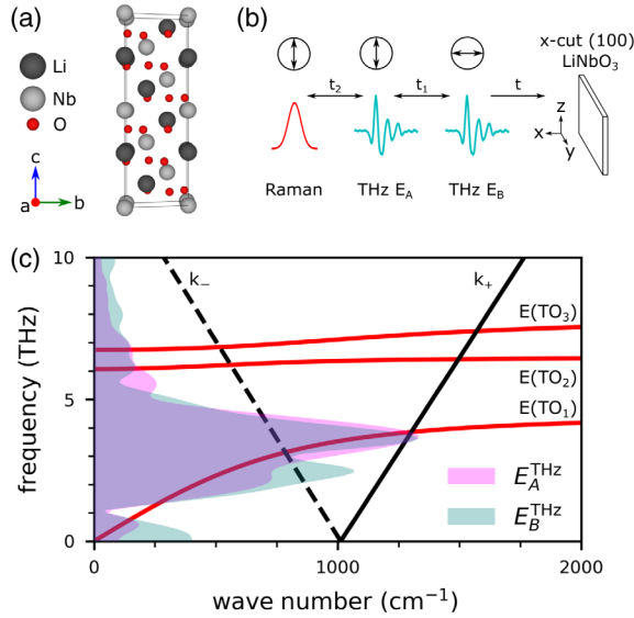
FIG. 1. (a) LiNbO 3 crystal structure in the hexagonal unit cell [33,34]. (b) Schematic of the 2D-TTR experiment, pulse sequence, and time definitions. The polarization of each pulse is indicated in the circles. Coordinates \{x, y, z\} refer to the crystal axes of x -cut LiNbO 3 , where x and z coincide with unit cell vectors a and c , and y is orthogonal to x and z . (c) Red: PHP dispersion curve for E -symmetry phonon modes [35]. Black: wave vector matching condition of the 800 nm probe for forward ( k + , solid) and backward ( k - , dashed) propagating PHPs [19]. The shaded regions show the THz bandwidth of E A THz and E B THz .
