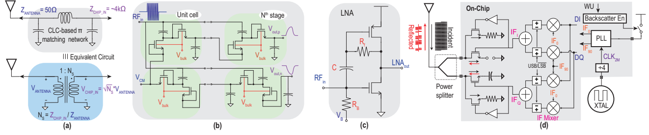
Figure 8: (a) CLC-based \pi matching network, (b) Schematic of passive pseudo-balun ED, (c) Schematic of LNA, (d) Transmission-line-less SSB QPSK Backscatter.
