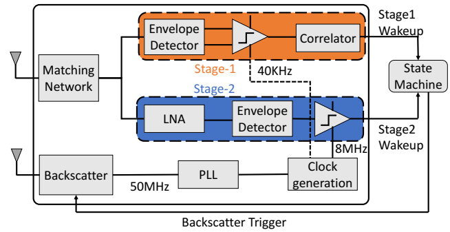
Figure 4: Design Overview of SyncScatter.
