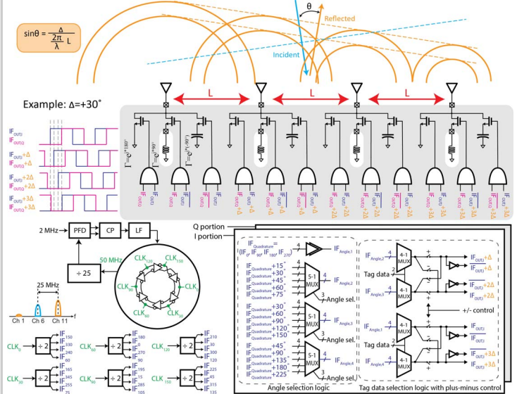
Figure 22.4.2: Schematic of the frequency and phase shifting beamsatter circuit enabling configurable beam steering for WiFi backscatter.
