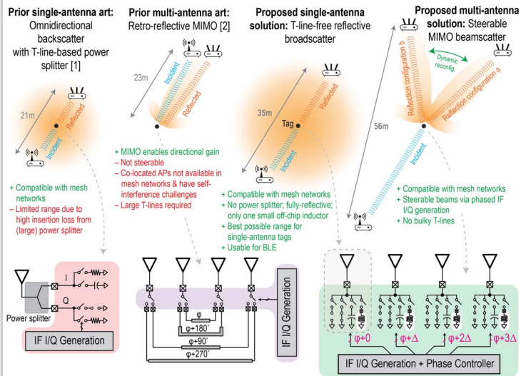
Figure 22.4.1: Prior-art omnidirectional and retro-reflective MIMO backscatter approaches (left); proposed transmission-line-free fully reflective broadside scattering and steerable MIMO directional beam scattering approaches (right).
