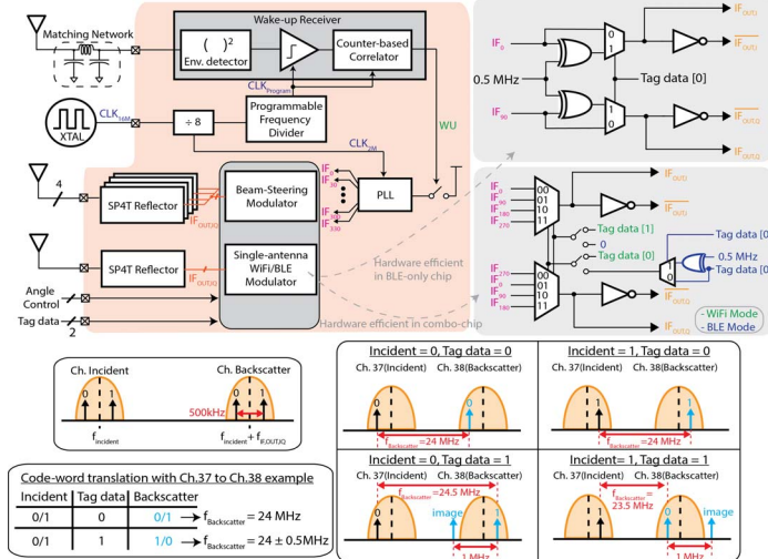
Figure 22.4.3: Overall system block diagram including a WiFi/BLE wake-up receiver, an on-chip multi-phase PLL, a multi-antenna WiFi beam steering block, and a single-antenna WiFi/BLE combo modulator (top); modulation and codeword translation scheme for BLE backscatter (bottom).
