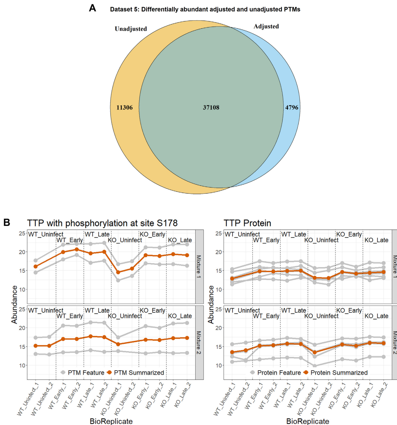
FIG. 7. Dataset 5: Mouse—phosphorylation—2mix-TMT, analysis with MSstatsPTM. A, the overlap of differential modified peptides for the PTM model with and without global protein level adjustment across all pairwise comparisons. B, comparing the profiling of protein TTP with the phosphorylation at site S178. The individual PTM and protein features are shown in gray, while the summarization is highlighted in red. The plots are separated according to TMT Mixtures 1 and 2. PTM, posttranslational modification; TMT, tandem mass tag.
