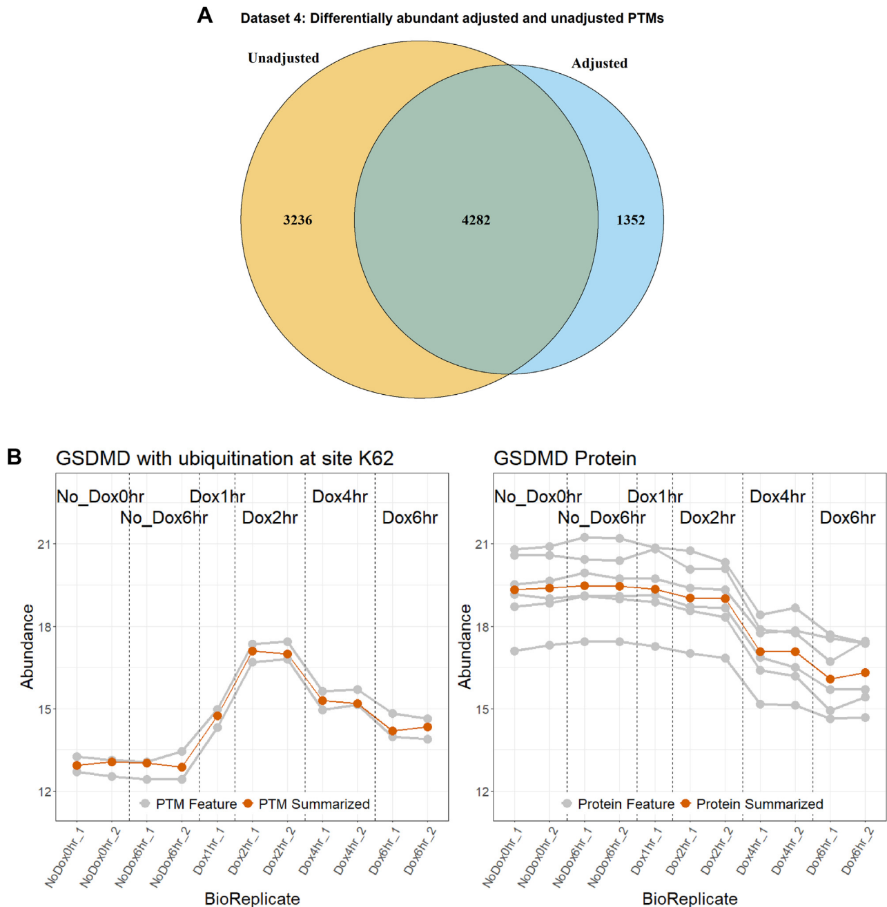
FIG. 6. Dataset 4: Human—ubiquitination—1mix-TMT, analysis with MSstatsPTM. A, the overlap of differential modified peptides for the PTM model with and without global protein level adjustment across all pairwise comparisons. B, comparing the profiling of protein GSDMD with the ubiquitination at site K62. The individual PTM and protein features are shown in gray, while the summarization is highlighted in red. GSDMD, Gasdermin D; PTM, posttranslational modification; TMT, tandem mass tag.
