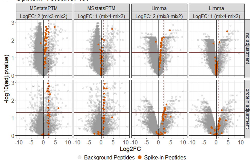
FIG. 5. Dataset 3: Spike-in benchmark—ubiquitination—label-free. A , the distribution of spike-in peptides log 2 -fold change estimated by MSstatsPTM, Limma, and ANOVA with and without adjustment. The expected log 2 -fold change is highlighted by a red 'X'. Protein adjustment removed systematic differences from the expected log 2 -fold change in all models. B , the statistical results of MSstatsPTM and Limma modeling the mix3-mix2 and mix4-mix2 comparisons before and after adjustment. The solid horizontal line shows the adjusted p-value cutoff of 0.05. The solid vertical line shows log 2 -fold change of 0. The dashed vertical line shows the expected log 2 -fold change of the spike-in peptides. Before adjustment, the spike-in peptides did not follow the expected log 2 -fold change but were more in line with expectation after adjustment.
