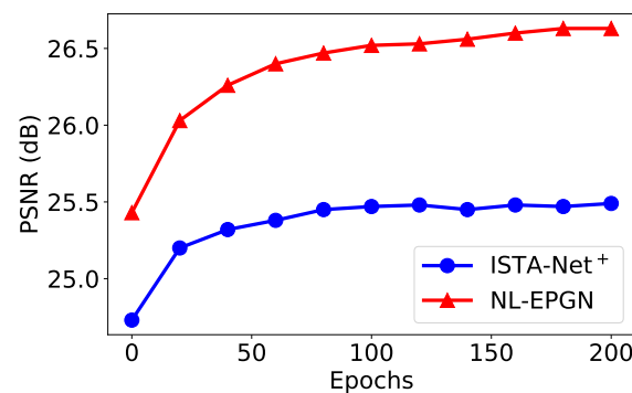
Figure 8. Average PSNR comparison between ISTA-Net + and NL-EPGN with various numbers of epochs during training with 3 phases on Set11 with a CS ratio of 10%.
