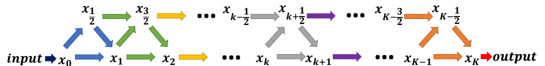
Figure 1. Overview of the K -phase extra proximal gradient network (EPGN) architecture. The arrows in the same color indicate computations within the same phase and share the same operators and parameters.
