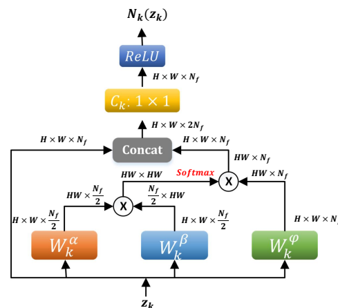
Figure 2. Data flow in the nonlocal operator \mathcal{N}_k (16). “ \otimes ” denotes matrix multiplication. Both input z_k and output \mathcal{N}(z_k) are of the same shape H \times W \times N_f (height \times width \times #channel) of the image.
