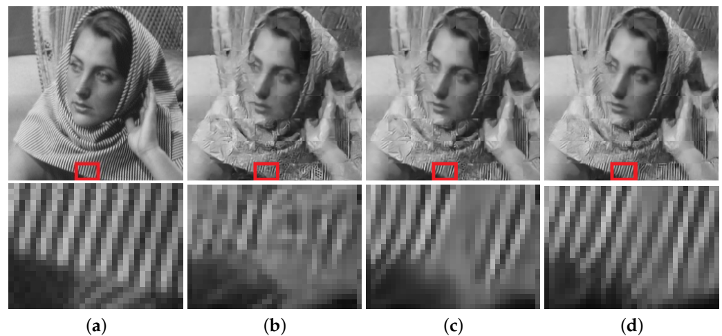
Figure 7. Reconstruction of the Barbara image with a CS ratio of 10% using the 9-phase ISTA-Net + (PSNR 23.59dB), 9-phase EPGN (23.89dB), and 7-phase NL-EPGN (24.27dB). (a) Ture. (b) ISTA-Net + . (c) EPGN. (d) NL-EPGN.
