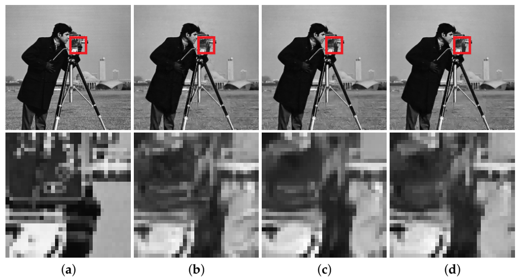
Figure 6. Reconstruction of the cameraman image with a CS ratio 25% using the 9-phase ISTA-Net + (PSNR 28.97dB), 9-phase EPGN (29.62dB), and 7-phase NL-EPGN (29.73dB). (a) Ture. (b) ISTA-Net + . (c) EPGN. (d) NL-EPGN.
