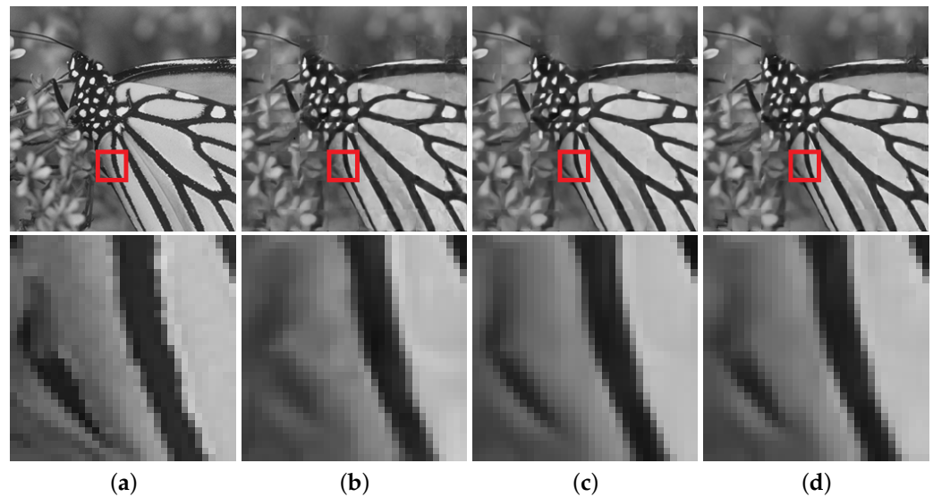
Figure 5. Reconstruction of a butterfly image with a CS ratio of 10% using the 9-phase ISTA-Net + (PSNR 25.91dB), 9-phase EPGN (26.47dB), and 7-phase NL-EPGN (26.58dB). (a) Ture. (b) ISTA-Net + . (c) EPGN. (d) NL-EPGN.
