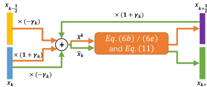
Figure 3. Data flow in the k th phase of EPGN. “ \oplus ” represents element-wise sum. Orange and green arrows represent computations in the first ((6a), (6b) and (11) with l = 1/2 ) and second ((6d), (6e) and (11) with l = 1 ) stages of EPGN, respectively.
