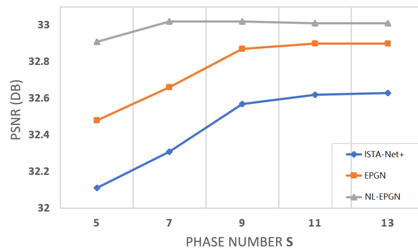
Figure 4. Average PSNR comparison between ISTA-Net + , EPGN and NL-EPGN with various phase number on image compressive sensing problem on Set11 with a CS ratio of 25%.
