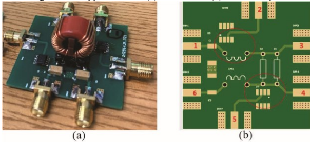
Fig. 7. EMI Filter board: (a) complete PCB, (b) Layout.
