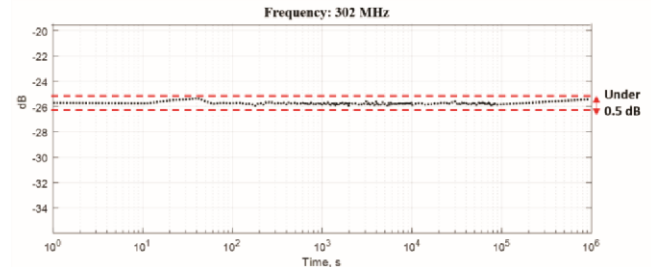
Fig. 8. Coupling from the EMI filter transformer to a pin of a nearby IC.
