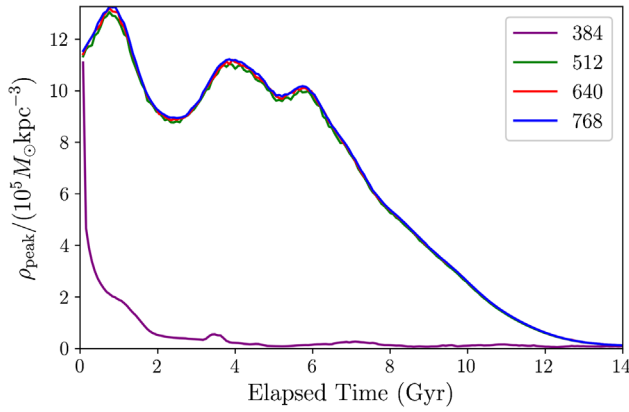
FIG. 8. The evolution of soliton peak density for different simulation resolutions, labeled by the number of grid cells per side. All simulations shown here use M_{\text{sol}} = 1.13 \times 10^8 M_\odot , x_c = 0.8 , and \tilde{\kappa} = -5.0 . The disruption times calculated at our fiducial resolution of 512 grid cells per side are stable at the 1% level for higher-resolution runs. Note that the peak density cannot be calculated meaningfully at a resolution of 384 grid cells per side because the maximum velocity criterion [Eq. (14)] is violated for this soliton and orbital configuration.
