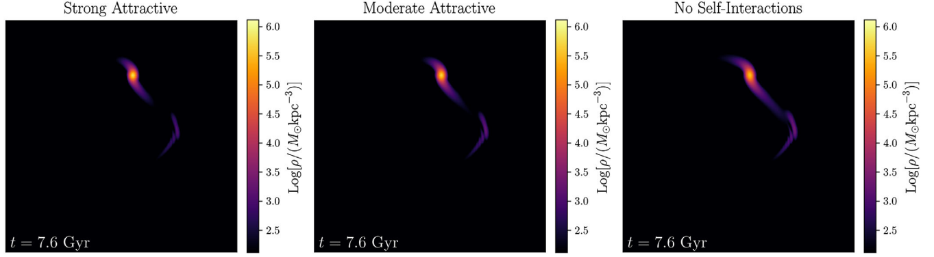
FIG. 10. Projected density distributions in the orbital plane from simulations where a soliton is tidally disrupted in the presence of attractive self-interactions with \tilde{\kappa} = -5.0 (left) and \tilde{\kappa} = -2.5 (center), and with no self-interactions (right). Note that the second density peak (i.e., the tidal tail of the stripped soliton) is increasingly coherent for stronger attractive self-interactions. In each simulation, the soliton mass is 1.13 \times 10^8 M_\odot and x_c = 0.8 .
