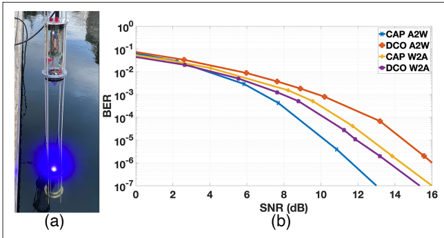
FIGURE 3. a) experimental setup and water-to-air communication for ocean experiments; b) BER analysis are conducted in coastal ocean water for both air-to-water (A2W) and water-to-air (W2A) configuration for CAP and DCO-OFDM modulation schemes.
