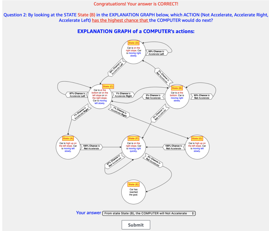
Figure 13: Second question of the user-study interface on AMT on the Mountain Car RL environment. The worker is asked to identify the next probable action that the RL agent would carry out given the current scenario of the car. If the worker incorrectly answers the first question (Figure 12), she/he will be informed with the correct abstract state of the explanation graph before answering this question.
