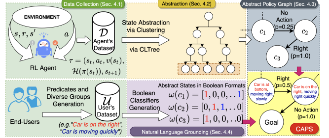
Figure 1: The overall architecture of the CAPS approach.
