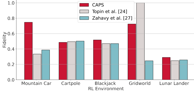
Figure 5: Fidelity for three baselines in the five baseline environments. Data was collected using a PPO policy.
