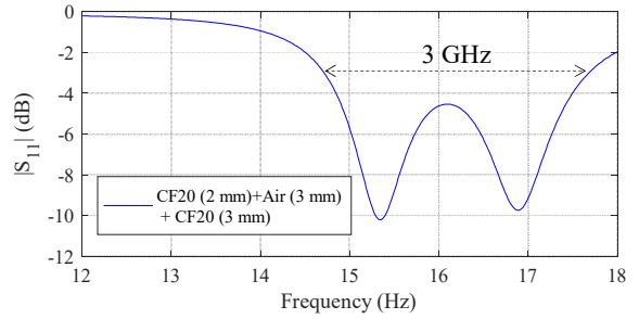
Fig. 6. Reflectivity/Reflection coefficient of the three-layer absorber.
