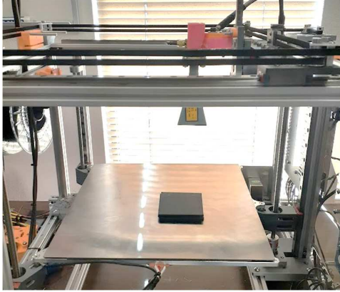
Fig. 8. Setup of the SAR reflectivity scan of the designed absorber.
