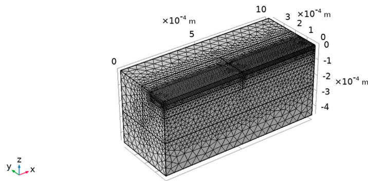
FIGURE 2 Meshed \text{Bi}_2\text{Te}_3 geometry used in our simulations.
