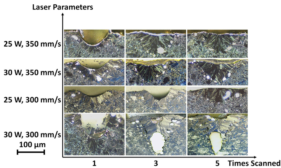
FIGURE 6 Polarized light microscopy images of the melt pool cross sections showing columnar dendritic grains.
