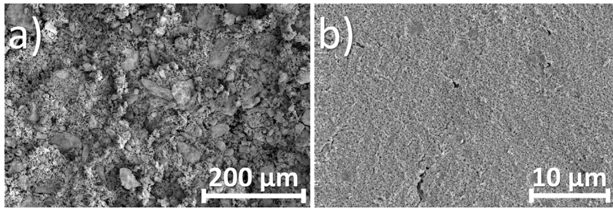
FIGURE 1 Scanning electron micrographs of (A) as-received \text{Bi}_2\text{Te}_3 powder and (B) cross section of the compacted \text{Bi}_2\text{Te}_3 powder prior to laser processing.
