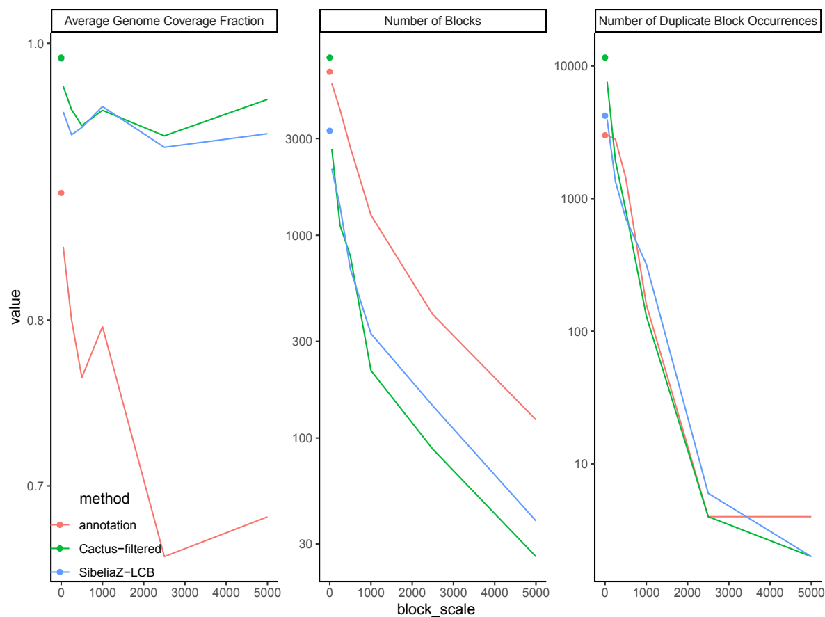
Fig. 2. maf2synteny Parameter Effects on Synteny Blocks. The effects of varying the ---block_sizes parameter of maf2synteny (default 5000) on the average genome coverage fraction, resulting number of synteny blocks, and the number of duplicate occurrences. The isolated points represent the values for the raw markers. Only methods used in our subsequent phylogenetic analyses are shown here, representing a single run configuration for each tool used to identify the raw syntenic markers that maf2synteny acts upon.
