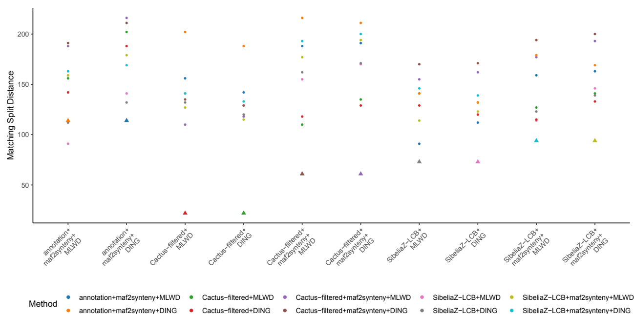
Fig. 6. Comparison of fully resolved MLWD and DING trees using Matching Split distance. As in Fig. 5, each point corresponds to the matching split distance between the method indicated at the x position and that denoted by the point's color. The MS distances between trees built from the same underlying syntenic blocks but using a different tree inference method are shown as triangular points. In the majority of cases, the trees closest to each other are in fact these pairs, with the exception of annotation+maf2synteny+MLWD having greater similarity to both trees from SibeliaZ-LCB+maf2synteny than to annotation+maf2synteny+DING. A comparison of annotation+MLWD to annotation+DING (without maf2synteny) cannot be shown due to the computational infeasibility of computing the distance matrix for the latter.
