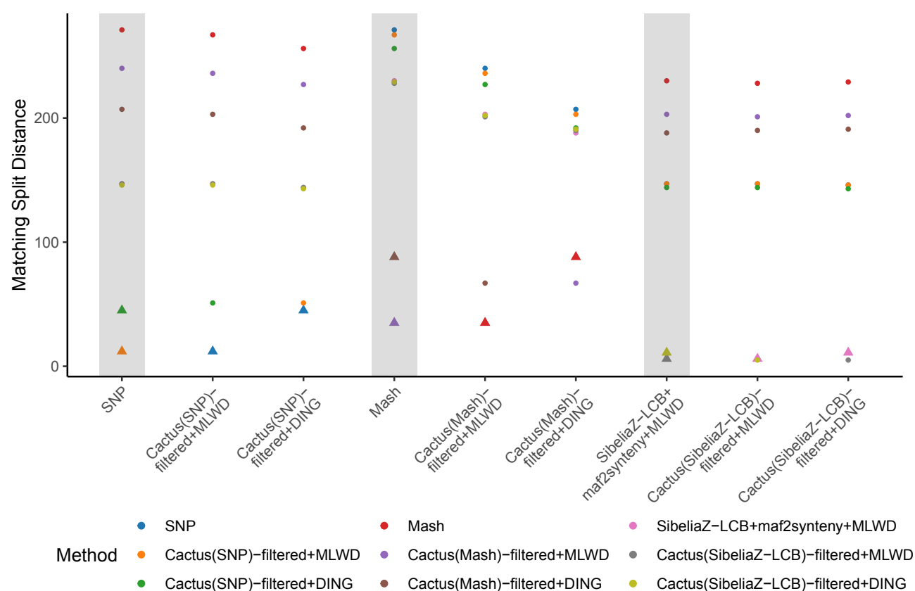
Fig. 5. Cactus whole-genome alignment is sensitive to the input guide tree. The plot shows matching split (MS) distances between rearrangement trees inferred from Cactus alignments based on 3 different guide trees: SNP, Mash, and Sibeliaz-LCB. Each point corresponds to the MS distance between the method indicated on the x-axis and that denoted by the point's color. The MS distances between MLWD/DING trees and the corresponding guide tree are shown as triangular points. The most similar tree to a given MLWD/DING tree is invariably either the guide tree used for the underlying Cactus alignment itself, or the tree built using the same synteny blocks but the other inference method (i.e. methodA+MLWD and methodA+DING). Furthermore, there is a large difference between these and the remaining independent Cactus results. The use of Sibeliaz-LCB+maf2synteny+MLWD as one of the guide trees further shows how Cactus can, to an extent, mimic another method's alignment and thereby produce a similar rearrangement tree.
