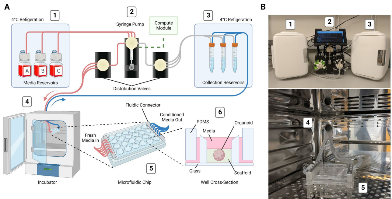
Figure 2. Design and implementation of the automated, microfluidic culture platform, the Autoculture . (A) Illustration of the automated, microfluidic organoid culture platform, the Autoculture . (B) Front view images of the Autoculture . (1) Refrigerator with reagent reservoirs. (2) Syringe pump, distribution valves, and control interface. (3) Refrigerator with conditioned media collection reservoirs. These components reside on a lab bench directly above the cell culture incubator. (4) Microfluidic tubes enter through an incubator port and connect to the (5) microfluidic well plate chip inside the incubator. (6) Cross-sectional diagram of a single well containing an organoid culture.
