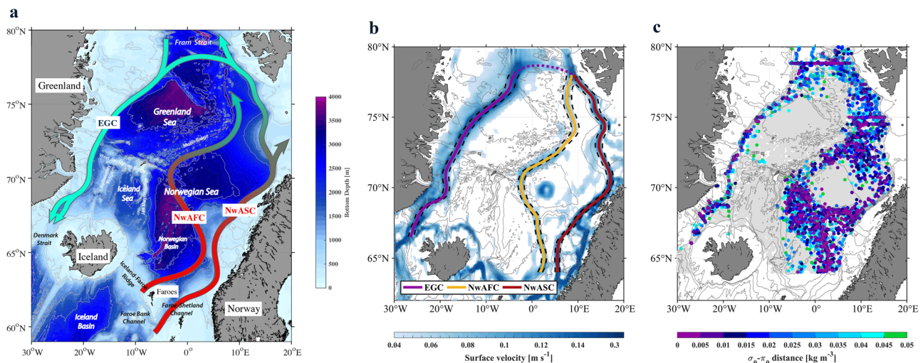
Fig. 1 | Pathways of Atlantic Water along the rim current system in the Nordic Seas. a Schematic circulation, modified from ref. 40 . The rim current system includes three boundary currents: the Norwegian Atlantic Slope Current (NwASC), the Norwegian Atlantic Front Current (NwAFC), and the East Greenland Current (EGC). b Composite of the long-term mean (2005–2018) sea surface velocity (absolute speed) from satellite observations and the GLORYS12 reanalysis product. The pathways of the three boundary currents in (b) were determined by maxima in the surface velocity field, shown by the solid lines. The black dashed lines denote
