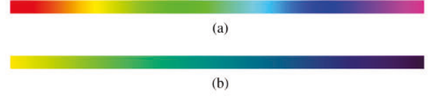
Fig. 2. (a) The gist_rainbow colormap is non-sequential and non-uniform. (b) The viridis colormap is sequential and uniform.
