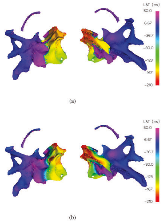
Fig. 12. Patient D, Map 6 interpolation by MAGIC-LAT (a) and GPMI (b) for m = 100 input LAT observations. The interpolations color the manifold surface underneath the known LAT observations. MAGIC-LAT very closely approximates the sharp early-meets-late transition region, while GPMI erroneously smooths it out with a wide blue to yellow transition band.
