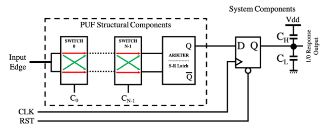
Fig. 1 Structure of an arbiter-PUF [14]. This includes both the PUF Structural Components as well as the Systems Components
