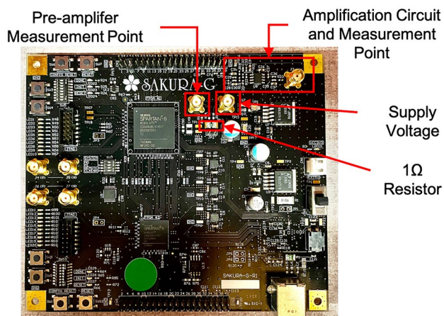
Fig. 6 Sakura-G FPGA development board [15]
