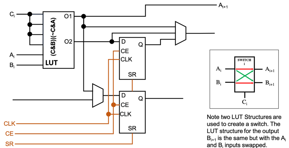
Fig. 3 Placement of a switch structure within the LUT components of a slice
