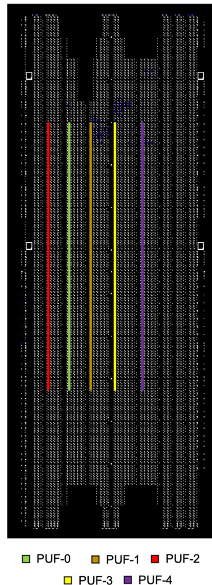
Fig. 7 Placement of the various PUF implementations within the fabric of the Sakura Development Board. The location of PUF-0, PUF-1, PUF-2, PUF-3, and PUF-4 are shown in green, orange, red, yellow, and purple colors, respectively
