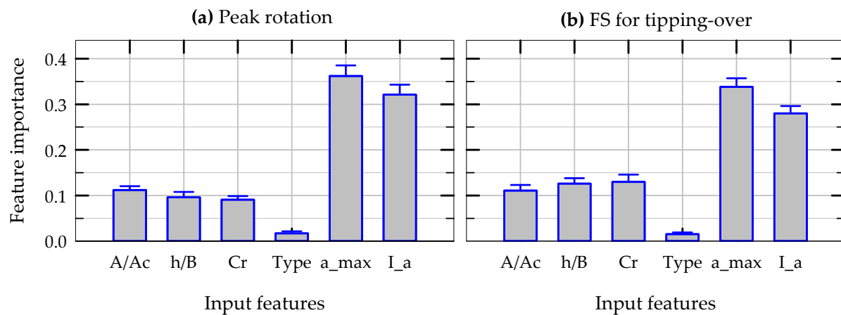
Figure 11. Results of mean (shown as boxes) and standard deviation (shown as error bars) of normalized feature importance scores for the prediction of (a) peak rotation and (b) factor safety for tipping over obtained from multiple RFR models.
