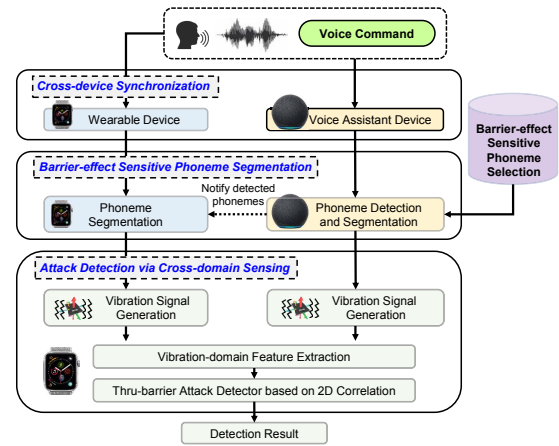
Fig. 5. System architecture.
