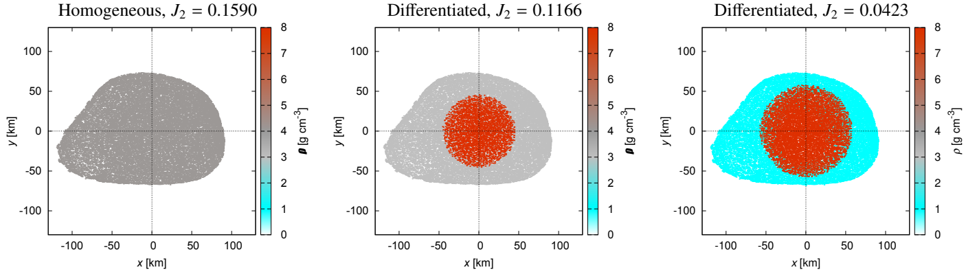
Fig. 3. Density profiles needed to obtain various J_2 values. The ADAM shape is used with fixed total mass m_1 = 7.78 \times 10^{18} kg. Left: Homogeneous body with \rho = 4.11 g cm ^{-3} , and nominal J_2 = 0.1590 . Middle: Differentiated body with iron core + silicate mantle ( \rho = 8 and 3 g cm ^{-3} ), and slightly lower J_2 = 0.1166 ; the core is spherical ( R \simeq 46 km) and the mantle irregular. Right: Extreme example with iron core + icy mantle ( \rho = 8 and 1 g cm ^{-3} ), and J_2 = 0.0423 (not realistic, however). The body is always plotted as a section with z < 0 to see its interior.
