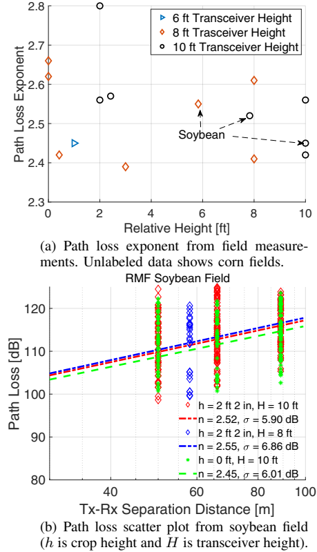
Fig. 2. Measurement results on path loss over crops.
