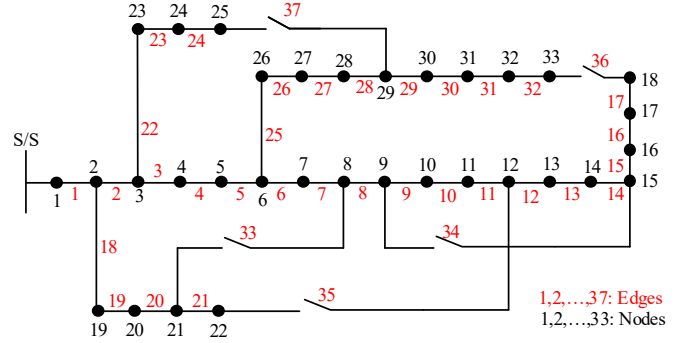
Fig. 1. 33-node distribution test system
