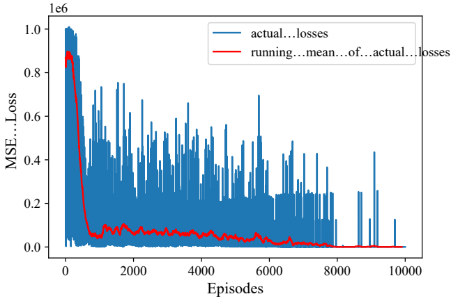
Fig. 3. MSE of losses of training episodes
