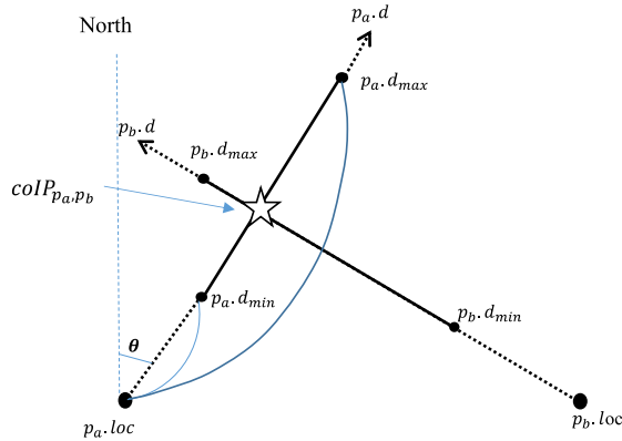
FIGURE 3. A cointeresting point between p_a and p_b .
