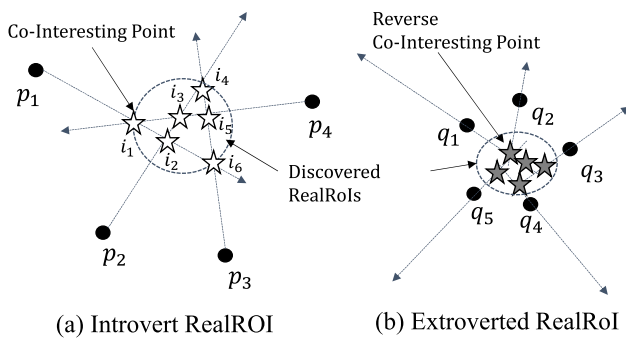
FIGURE 2. Examples of introverted and extroverted ROIs.
