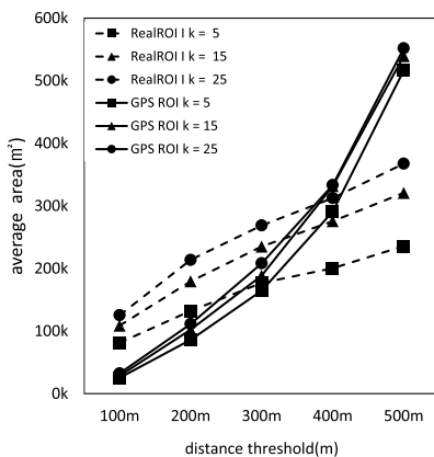
FIGURE 6. Effect of the distance threshold ( \varepsilon ).
