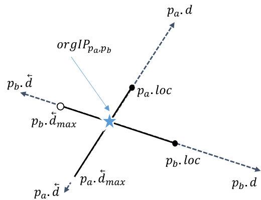
FIGURE 5. An interesting origin point between p_a and p_b .
