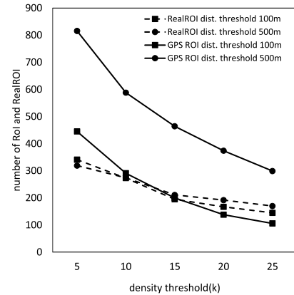
FIGURE 7. Effect of the density threshold ( k ).
