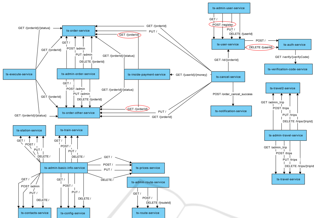
Figure 2: The communication diagram from manual analysis of the benchmark. Elements not found by Prophet circled in red.
