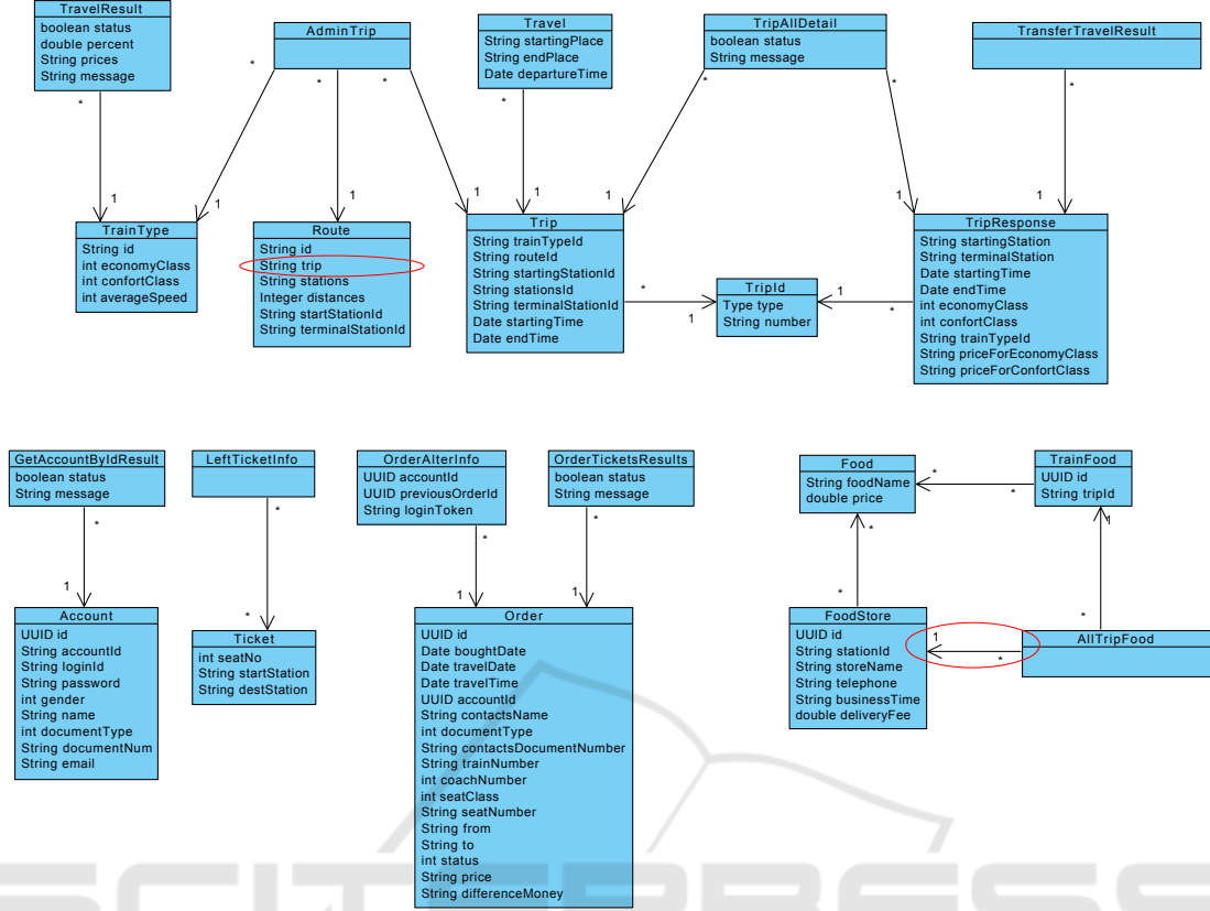
Figure 1: The class diagram from manual analysis of the benchmark. Elements not found by Prophet circled in red.
