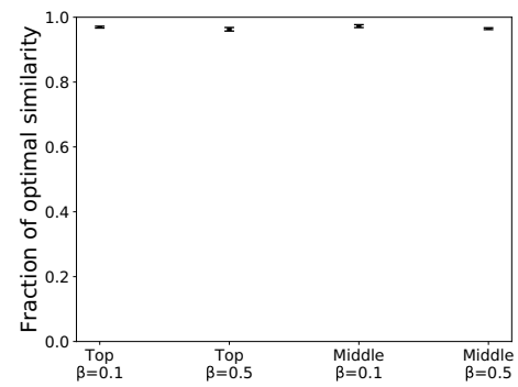
(b) Second-stage papers chosen as the top- or middle-scoring papers from ICLR
