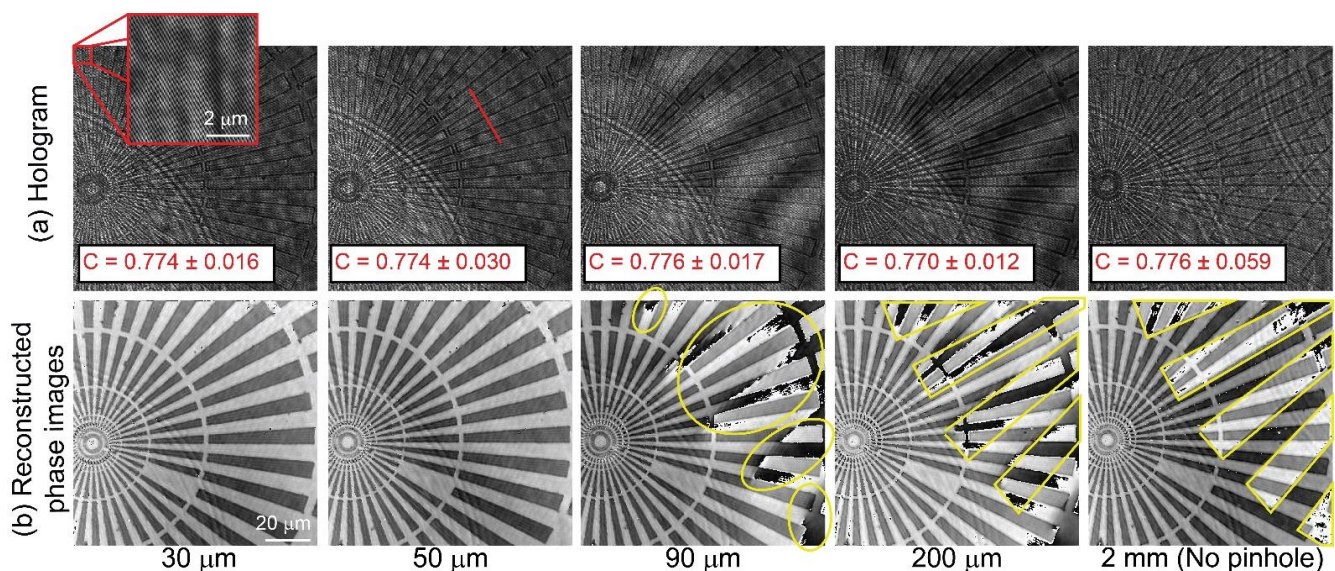
Figure 3. Evaluation of the pinhole size in the FB-based DHM system: (a,b) Experimental holograms and reconstructed phase images of the star pattern for different pinhole sizes. The inset in panel (a) shows the interference pattern created by the FB. The value of the fringes' contrast estimated along the red direction (red font) is shown in panel (a).
