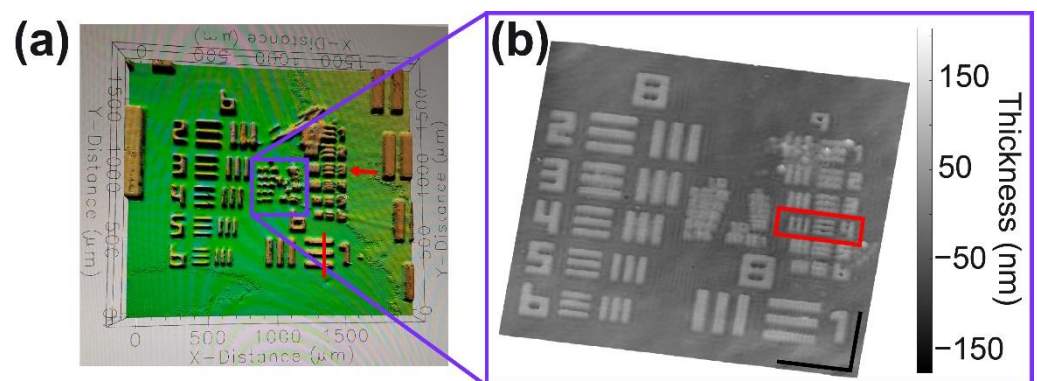
Figure 6. Reflective high-resolution USAF 1951 target imaged with (a) a profilometer and (b) the proposed common-path DHM operating in reflection mode. The scale bars in panel (b) are 14.4\ \mu\text{m} . The red rectangle in panel (b) refers to the smallest resolvable element of the USAF target.
