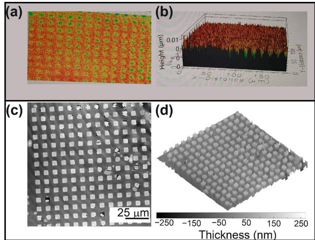
Figure 7. Reflective array printed in the logo of Photomask Portal. Thickness maps results obtained with (a,b) a profilometer and (c,d) the proposed common-path DHM operating in reflection mode.
