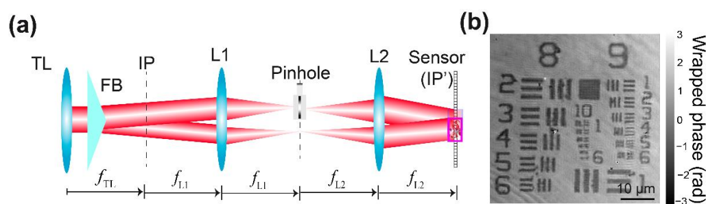
Figure 2. (a) The optical configuration of the proposed common-path DHM using a Fresnel biprism and a spatial filtering system to create the interference pattern between the complex amplitude distribution scattered by object and imaged by the system and a uniform reference wave. (b) Reconstructed phase image of a USAF target from the QPM target.
