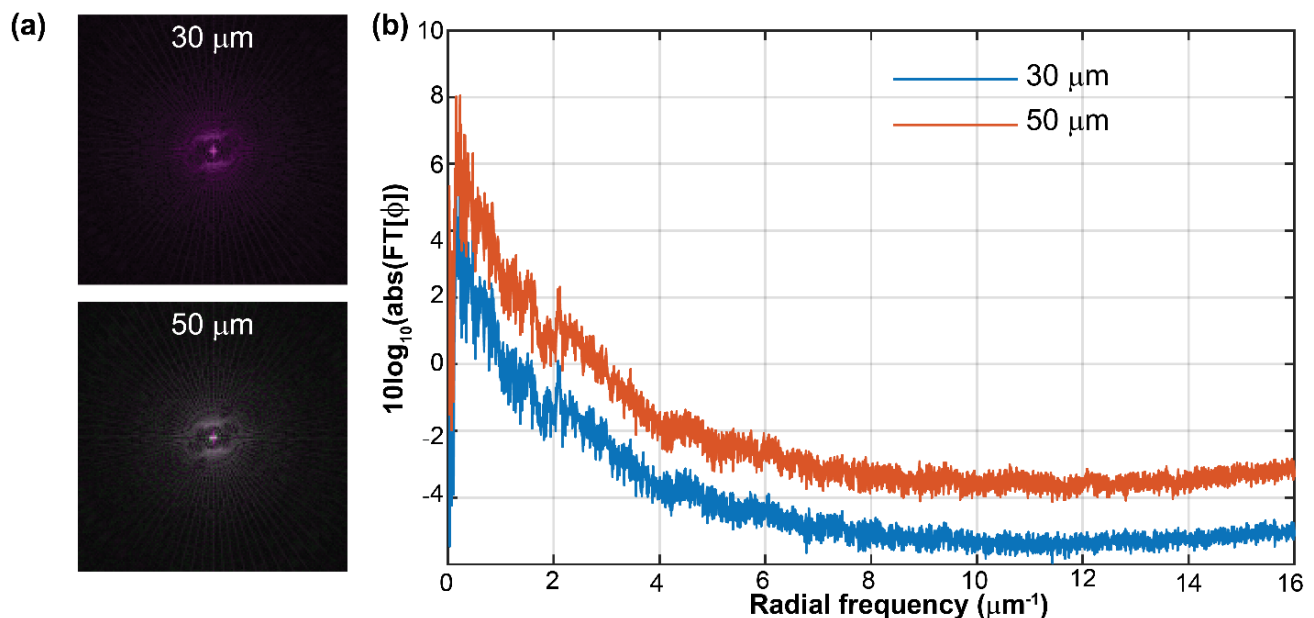
Figure 4. Comparison of the Fourier spectrum of the reconstructed phase images for a pinhole size of 30 and 50 \mu\text{m} in the FB-based DHM system. (a) The 2D Fourier transform of the reconstructed phase images for the pinholes of 30 and 50 \mu\text{m} . (b) Power spectrum distribution versus the radial frequency for both pinholes.
