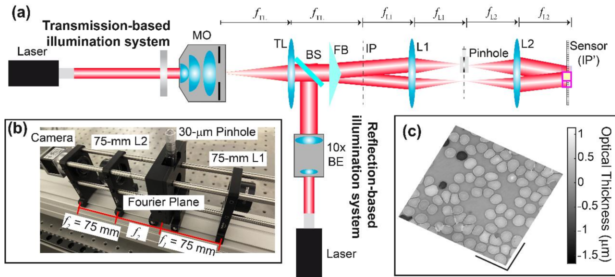
Figure 5. (a) The optical configuration of the dual-mode common-path digital holographic microscopy using a Fresnel biprism for quantitative phase imaging of transmissive and reflective samples. (b) Experimental setup of the compact QPI module with a spatial filtering system to generate a uniform reference beam. (c) Three-dimensional distribution of the optical thickness of human RBCs using the transmission-based illumination system. The scale bar is 25 μm.
