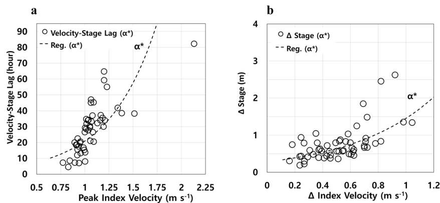
Fig. 2 Parameterized velocity-stage peak correlations. a Index-velocity vs. stage peak lag and b index-velocity gradient vs. associated stage peak gradient. Note: the unsteadiness coefficient, \alpha^* , is determined with Eq. (4) applied to the 2014–2018 training dataset (see the “Methods” section and Supplementary Data 3).
