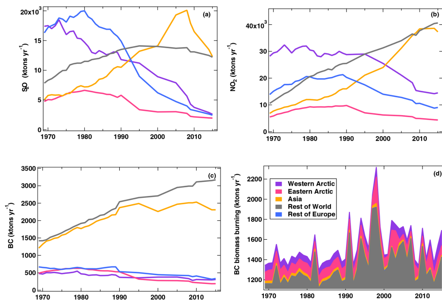
Figure 4. Anthropogenic emissions of SO 2 (a), NO 2 (b), BC (c) and BC from biomass burning (d). Anthropogenic emissions are based on ECLIPSE v6B (Höglund-Isaksson et al., 2020). Data from before 1990 are based on CMIP6 (Hoesly et al., 2018; van Marle et al., 2017) scaled linearly to match ECLIPSE v6B. Biomass burning data are from CMIP6. The Western Arctic region refers to the following countries: USA and Canada; Eastern Arctic region: Kingdom of Denmark, Finland, Iceland, Norway, the Russian Federation and Sweden. The grouping follows the report of the Arctic Monitoring and Assessment Programme on short-lived climate forcers and refers to entire countries (AMAP, 2021).
