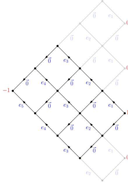
Figure 4.3: GT(1, 1, 1, 0, 0) and the associated map gwt .
