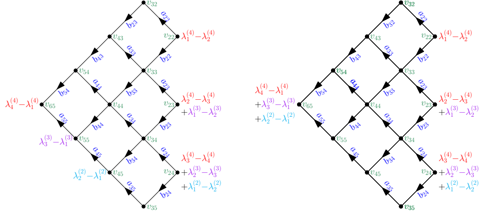
Figure 4.4: The flow networks G(\lambda^{(1)}, \lambda^{(2)}, \lambda^{(3)}, \lambda^{(4)}) (left) and \widehat{G}(\lambda^{(1)}, \lambda^{(2)}, \lambda^{(3)}, \lambda^{(4)}) (right). Vertices without netflow indicated have netflow 0.
