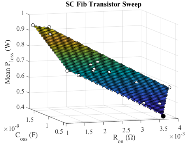
Fig. 14. Switched capacitor Fibonacci transistor design space where all converter transistors are the same. The optimal point, shown by the black circle, is the EPC2055 transistor. P_{loss} is a weighted mean of hundreds of simulations for each transistor between the input voltage and output power range.
