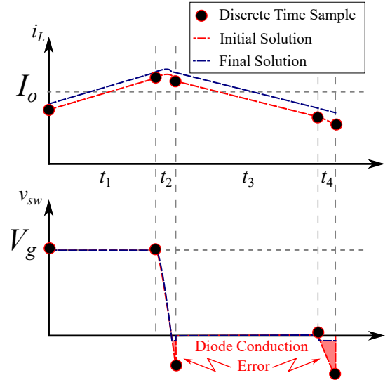
Fig. 4. Waveform of a synchronous buck converter after the high side device turns off. The initial guessed dead time length is too long between active switching actions.
