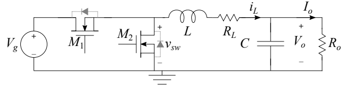
Fig. 2. Synchronous buck converter used in Fig. 1 and Fig. 4.
