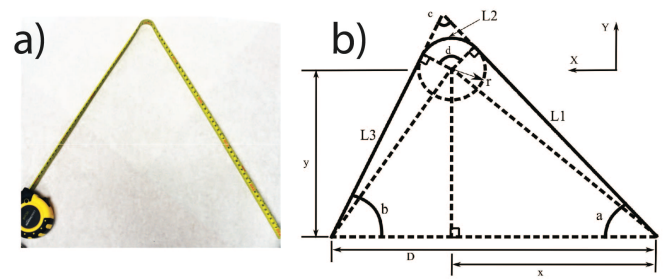
Fig. 2. a) Example of a tape spring with a single bend in the middle. b) Geometric modeling of the tape fin.
