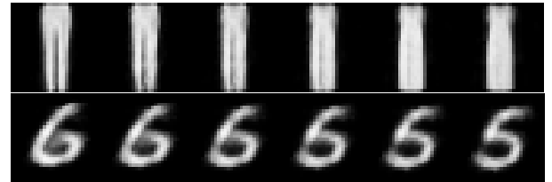
Fig. 3. Images generated when moving from one cluster to another within a projection, and feeding the x and y coordinates into NNInv. Top row: FashionMNIST, moving from class “pants” to class “dress”; bottom row: MNIST, moving from class 6 to class 5.
