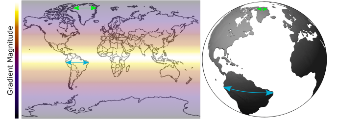
Fig. 7. Two equal length line segments (green and blue) are placed on a Mercator projection of the Earth overlaid with its gradient image. After inverse projection, the lengths of these segments are dramatically different. The degree of change corresponds to the difference in the pseudo total derivative, shown by the gradient image overlay in the projection. Note that the green segment (in a region of low gradient) shrinks vs the blue segment (in a high gradient region around the equator). This figure is an illustrative example of how gradient images function (note that the figure does not reflect the actual gradients of the sphere).
