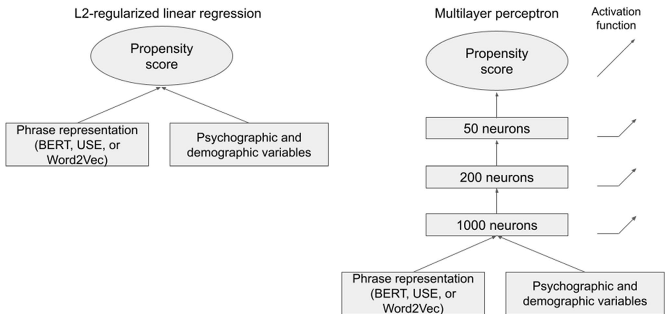
Fig. 3 Behavioral propensity predictive models. To predict behavioral propensity ratings, we used phrase representations—from BERT, USE, or Word2Vec—and participant demographic and psychographic
