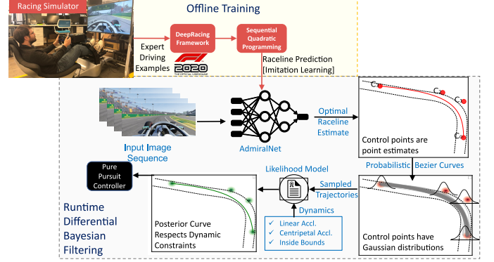
Fig. 1. The key idea in Differential Bayesian Filtering is that we fit Gaussian distributions over a Bézier curve's control points to generate a distribution of trajectories that respect the ego vehicle's dynamic limits.
