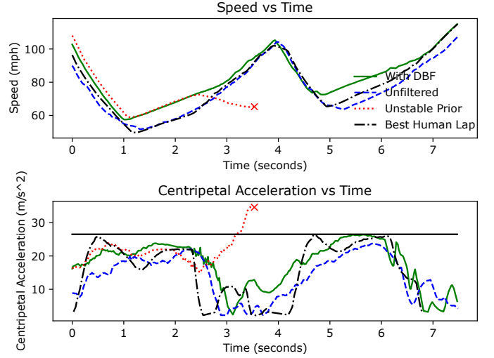
Fig. 6. Our artificially accelerated prior is dynamically infeasible and causes the car to spin out on the Turn3-Turn4 chicane. Differential Bayesian Filtering brings that prior back within the car’s physical limits. Our specified dynamic limit of 26.5[m/s^2] is marked on the lower plot. Our approach pushes the car right up to its dynamic limit, but does not exceed it. For the unstable prior, both plots end at the point the car spins out.
