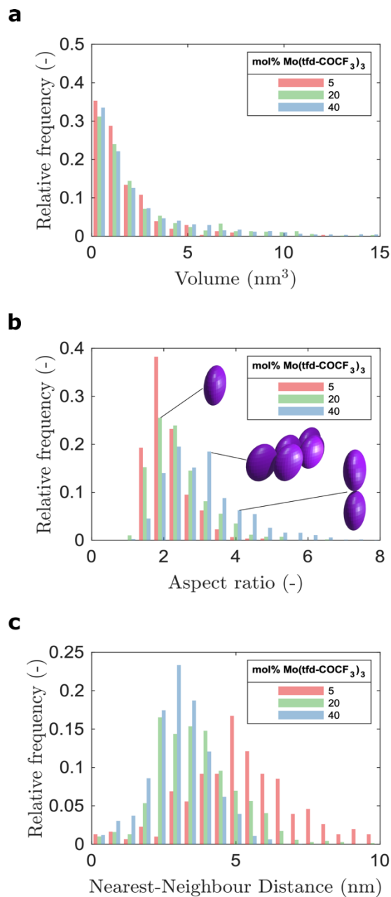
Figure 4: Histograms from data analysis including all clusters in a volume equivalent to an in-plane area of 150 nm by 150 nm for each sample, displaying distribution of (a) cluster volume, (b) cluster aspect ratio and (c) nearest-neighbour cluster distance. Examples of dopant cluster conformations for different aspect ratios are illustrated as insets in (b).
