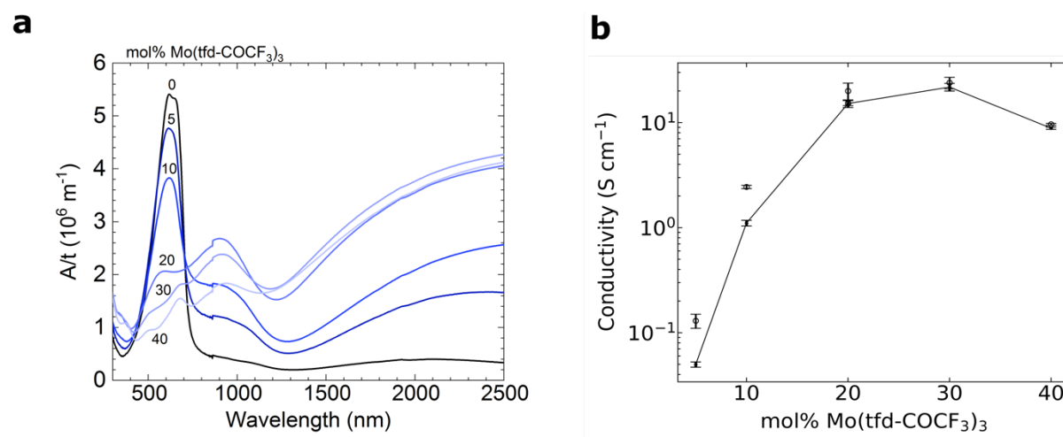
Figure 5: (a) UV-Vis-NIR absorbance spectra with the measured absorbance A normalised by the film thickness t . (b) Electrical conductivity of 40-90 nm thick films of \text{p}(\text{g}_4\text{2T-T}) doped with \text{Mo}(\text{tfd-COCF}_3)_3 ; average values and errors were obtained by measuring one sample for each dopant concentration five times and calculating the mean and standard deviation. The reproducibility of samples was confirmed by repeating the measurements on independently prepared films (Figure S3 and open symbols in Figure 5b).
