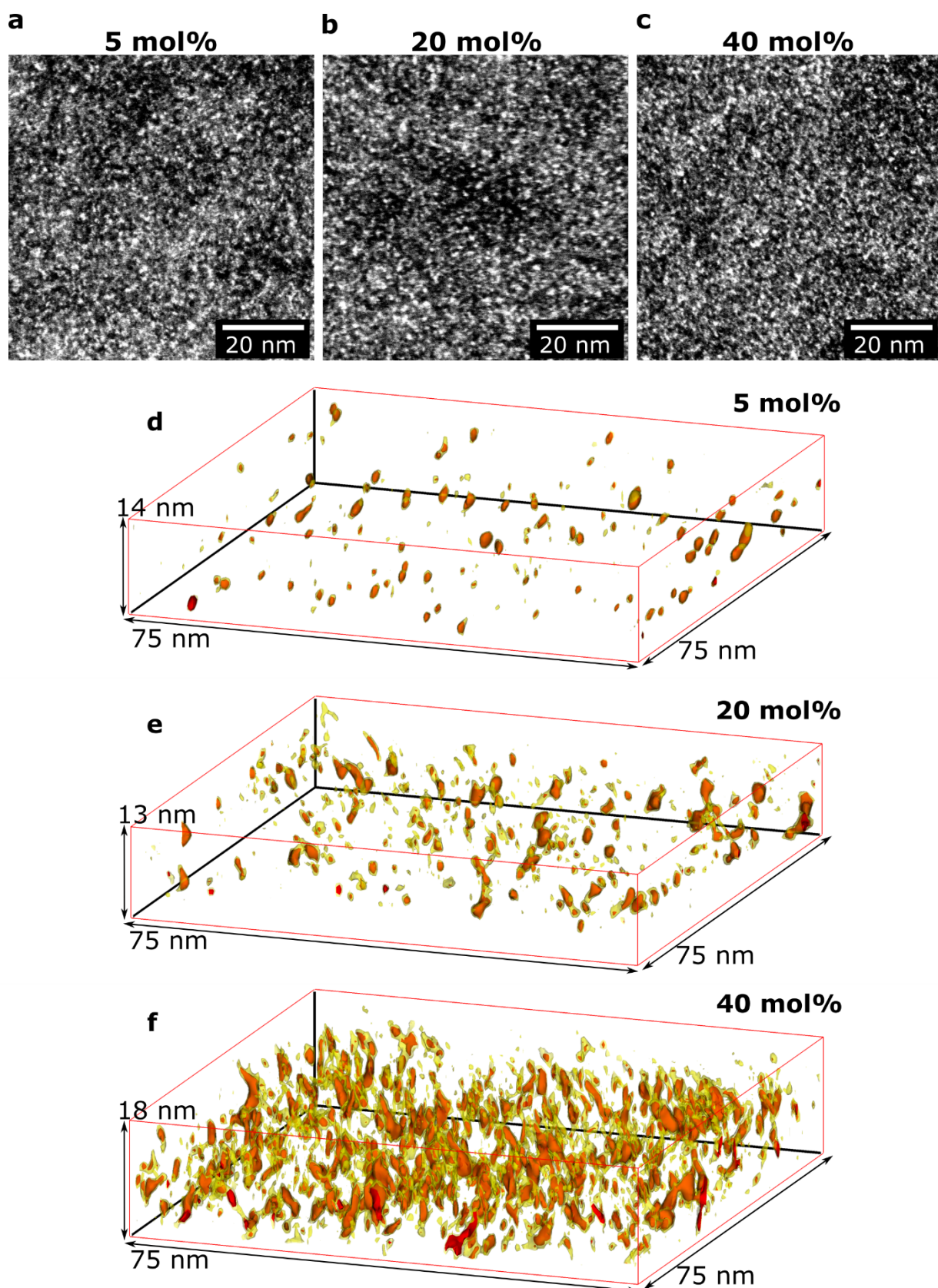
Figure 2: Electron microscopy (a-c) HAADF-STEM images of representative areas and (d-f) tomography reconstructions of p(g42T-T) doped with 5, 20, and 40 mol% Mo(tfd-COCF 3 ) 3 , respectively. The sizes of the volumes are marked in nm. Red intensity thresholds in the reconstructions were chosen in order to visualise the position of Mo(tfd-COCF 3 ) 3 species. A lower intensity threshold is displayed in yellow.
