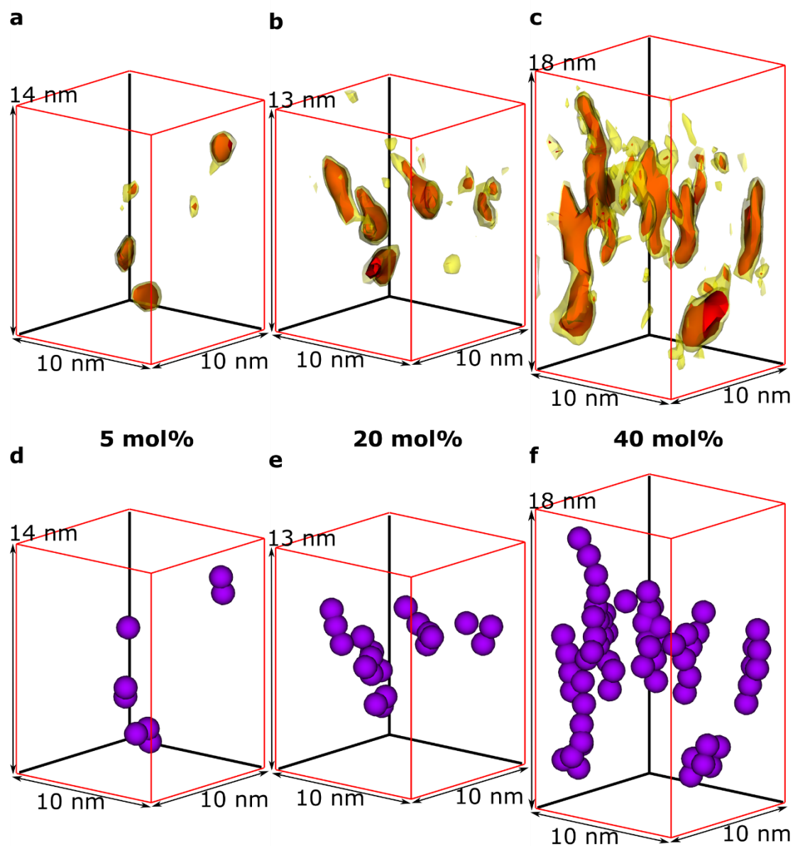
Figure 3: Representative sub-volumes of the tomographic reconstructions of p(g42T-T) doped with 5, 20, and 40 mol% Mo(tfd-COCF 3 ) 3 , respectively. (a-c) Reconstructed sub-volumes showing the clusters and (d-f) markers indicate the positions of individual Mo(tfd-COCF 3 ) 3 species in the clusters and visualise the gradual change in cluster morphology.
