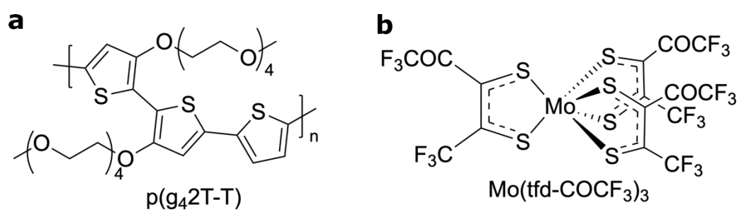
Figure 1: Molecular structures of (a) the polymer p(g_42T-T) and (b) the molecular dopant Mo(tfd-COCF_3)_3 .
