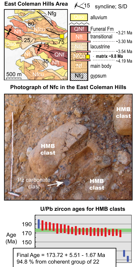
Figure 5. Diagrams show details of the East Coleman Hills area. Mapping and stratigraphy are after McAllister (1970) and Knott et al. (2018), respectively. HMB—Hunter Mountain Batholith; Nfc/m/u—lower/middle/upper conglomerate of the Furnace Creek Formation; Qao—Quaternary alluvium; QNF—Neogene–Quaternary Funeral Formation; Nft—transitional member of Furnace Creek Formation; Nfg—gypsum member of Furnace Creek Formation.
