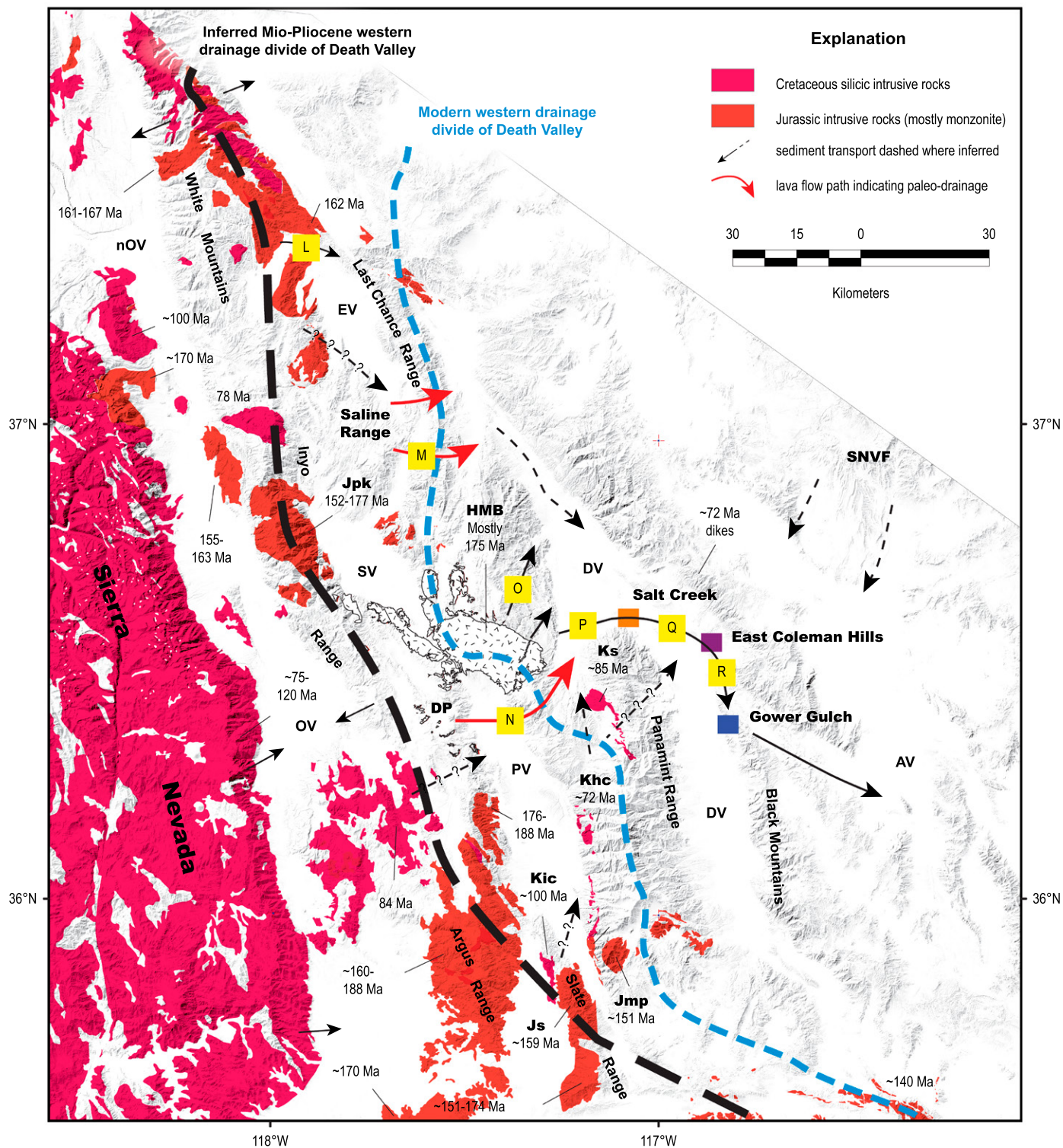
Figure 11. Map shows the distribution and ages of Jurassic and Cretaceous plutons and batholiths in the study area. The pathways with letters in yellow boxes are in Figure 2 and Table 2. Note the location of the modern (blue dashed line) versus inferred Mio-Pliocene (thick black dashed line) western drainage divide for Death Valley (DV). Mapping is from compilation of Lutz et al. (2017). Most ages are from the NAVDAT database. The following probable contributors to the age spectra in Figure 10 are shown in bold font. Kic—Isham Canyon quartz monzonite (Andrew, 2022); Ks—Skidoo granite (Barba, 2020); Khc—Hall Canyon pluton (Mahood et al., 1996); Jmp—Manly Peak quartz monzonite (Andrew, 2022); Js—Stockwell diorite (Dunne and Walker, 2004; Andrew, 2022); SNVF—Southwest Nevada Volcanic Field; AV—Amargosa Valley; EV—Eureka Valley; OV—Owens Valley; PV—Panamint Valley; SV—Saline Valley. Jpk—Jurassic Pat Keys pluton; Dp—Darwin Plateau; nOV—northern Owens Valley; HMB—Hunter Mountain Batholith.
