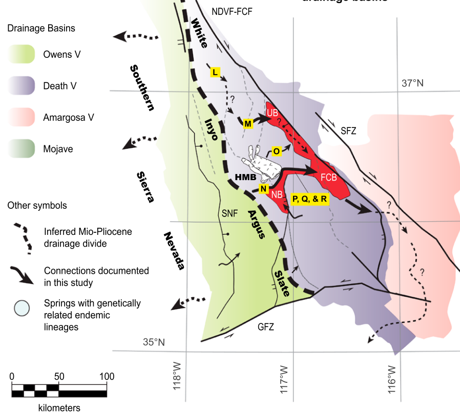
Figure 15. Map-view reconstruction shows (A) Pliocene drainage basins that predated (B) the modern, endorheic subbasins of the southwestern Great Basin. Reconstructed locations of faults in panel A are simplified from Lutz et al. (2022). Grey dashed lines in panel A are faults that accrued the most slip after ca. 4 Ma and formed much of the modern Basin and Range topography. Letters “L, M, R, etc.,” refer to constraints documented in other figures and in the text. The red areas indicate the interconnected northern and southern fluvial courses. FCB—Furnace Creek Basin; NB—Nova Basin; UB—Ubehebe Basin; BMF—Black Mountains fault zone; EIF—East Inyo fault zone; GFZ—Garlock fault zone; HMB—Hunter Mountain Batholith; HMF—Hunter Mountain fault zone; NDVF-FCF—Northern Death Valley–Furnace Creek fault zone; OVF—Owens Valley fault zone; PV—Panamint Valley; SFZ—Stateline fault zone; SNF—Sierra Nevada frontal fault zone; WMF—White Mountains fault zone; DV—Death Valley; SR—Saline Range.
