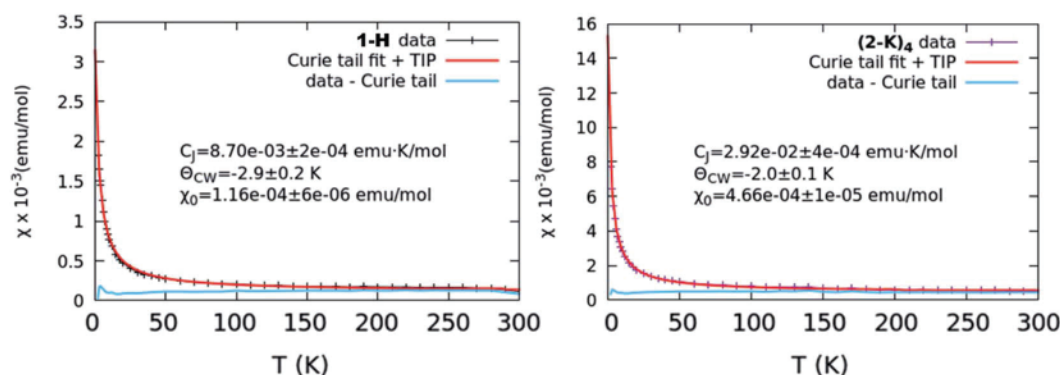
Fig. 5 \chi vs. T curves representative of the lowest level of TIP (left, 1-H) and greatest level of TIP (right, (2-K) 4 ). In both cases, the collected curve is shown along with the results from a Curie–Weiss fit as well as the data with the Curie tail subtracted. Other collected curves and fits are shown in Fig. S17.†
