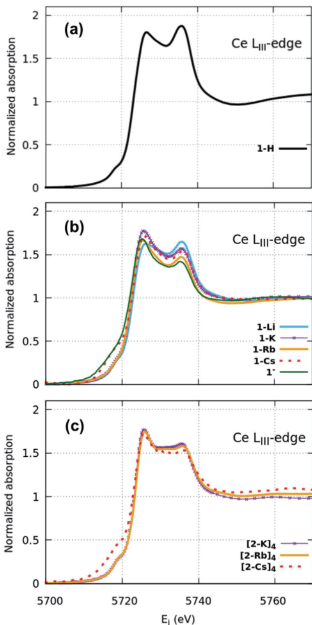
Fig. 2 Ce L III edge XANES spectra of the (a) anilide 1-H, (b) imido 1-M and (c) oxo (2-M) 4 samples. Each sample features the doublet peak characteristic to formal Ce(IV) but with differences in line shape. Increased amplitude below 5720 eV in the 1-Cs, 1 − , and [2-Cs] 4 data is due to the Cs L I edge.
