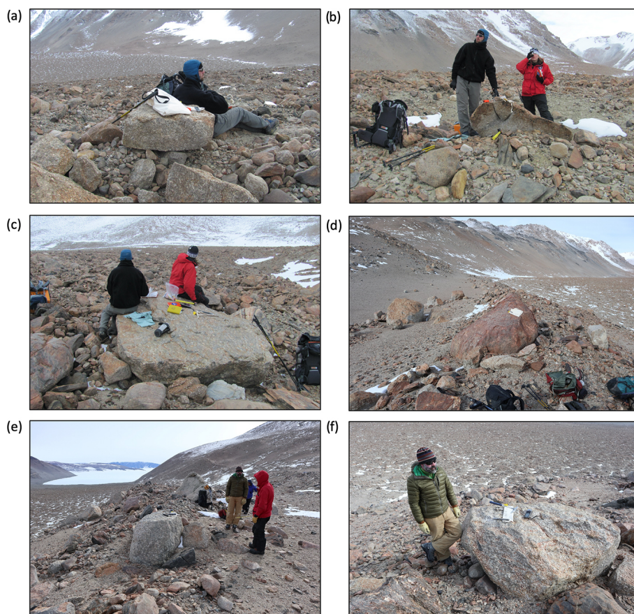
Figure 4. Photographs of surface boulders sampled from (a–c) the Middle drift surface and (d–f) the east lateral moraine; (a) 11-OV-ER-117, (b) 11-OV-ER-118, (c) 11-OV-ER-119, (d) 17-OV-ERR-213, (e) 17-OV-ERR-217, and (f) 17-OV-ERR-218.
