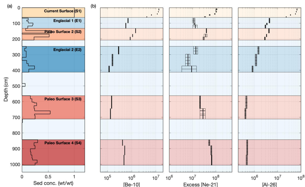
Figure 7. Depth plot of (a) sediment concentration (weight sediment/weight sediment and ice) and (b) measured ^{10}\text{Be} , ^{26}\text{Al} , and ^{21}\text{Ne} nuclide concentrations. The bold vertical lines represent the average measured cosmogenic nuclide concentrations in the samples. The width of the surrounding black boxes shows the measured uncertainty in the cosmogenic nuclide concentrations, and the horizontal black lines indicate the original ice core segments and are the same for all three nuclides. Color shades highlight the source of the debris. Yellow depicts the current supraglacial debris samples (S1) and has same origin as blue samples (E1 and E2) identified as “englacial debris” having no prior surface exposure before being subglacially entrained. Samples in shades of red are identified as “paleo-surfaces” (S2, S3, and S4) and are made of recycled surface debris that was exposed on the surface and entrained as the glacier overrode previously ice-free areas as it advanced into Ong Valley.
