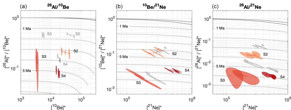
Figure 10. Paired-nuclide diagram for (a) ^{26}\text{Al} – ^{10}\text{Be} , (b) ^{10}\text{Be} – ^{21}\text{Ne} , and (c) ^{26}\text{Al} – ^{21}\text{Ne} pairs. Solid black lines show the steady-state erosion zone, and dashed lines show the burial lines as million-year decay isochrons. The nuclide concentration for each data point is represented by a shaded ellipse of its 1\sigma uncertainty. Grey data points show the measured nuclide concentrations for the paleo-surface samples as described in Fig. 9d–e. Shaded red data ellipses show the resulting nuclide concentrations when subtracting the modeled nuclide concentration from the measured. The burial age (dashed isochron lines) for which a sample lies represents the apparent burial age and is the maximum single period the sample has been buried since current time. Color shades refer to the different paleo-surface units as described in Fig. 7. * signifies nuclide concentrations normalized to respective surface production rate.
