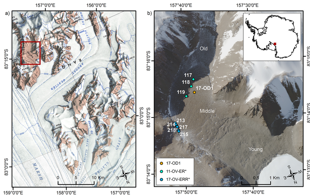
Figure 1. Location of Ong Valley. (a) Cropped USGS 1 : 250 000 scale topographic map of Miller Range, Antarctica, showing the location of Ong Valley. The red rectangle indicates the location of Ong Valley opening perpendicular to Argosy Glacier. (b) WorldView 2 satellite image of Ong Valley, Antarctica (© 2016 Maxar). The dots indicate sampling sites for pit and ice core (orange), Middle drift surface boulders (cyan), and lateral moraine boulders (blue). The legend shows the prefixes of sample names.
