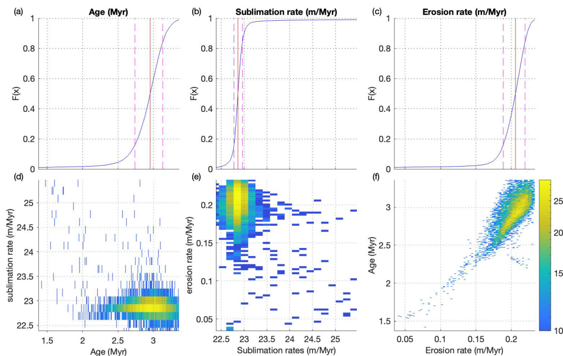
Figure 8. (a–c) Cumulative distribution of 10 000 fitted Monte Carlo simulation results showing the 50th percentile (red line) with error bounds given by the 16th and 84th (pink lines). (f–e) Density plot as paired distribution of Monte Carlo simulation results separated into 1000 bins with yellow being high density and blue low density. Both the vertical and horizontal axes (d–f) are truncated to the 98 % (0.01 and 0.99) confidence interval.
