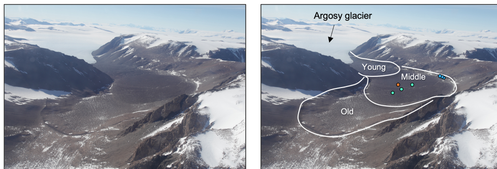
Figure 2. Oblique aerial photograph of Ong Valley (left) with added markings (right) indicating the Young, Middle, and Old drifts (Bibby et al., 2016). The photograph is looking northward and down-valley. The dots represent the sampling sites as identified in Fig. 1.
