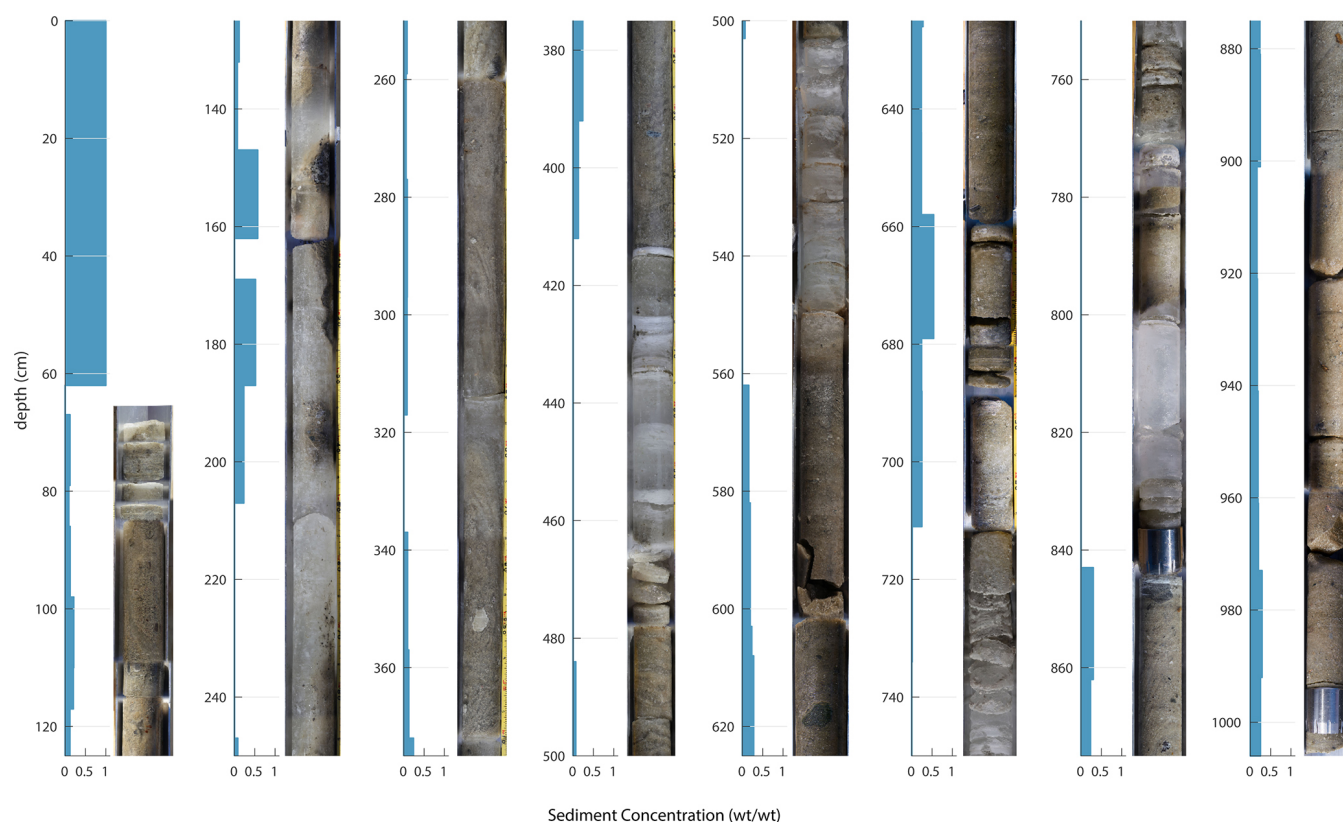
Figure 5. Image of the 17-OD1 ice core. The full image is stitched together from multiple individual pictures each covering approximately 20 cm of core length. The blue graph shows the corresponding debris concentration calculated by weight at depth below the surface. The topmost 62 cm is the thickness of the overlying supraglacial debris layer (not shown in pictures). See the complete ice core image in the Supplement.
