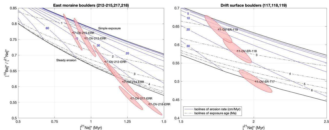
Figure 11. ^{10}\text{Be} – ^{21}\text{Ne} paired-nuclide diagram of the boulder samples. Solid black lines are the simple exposure line and steady-state erosion line, which marks the zone of continuous exposure. Blue lines are isolines of constant steady erosion ( \text{cm Myr}^{-1} ), and dashed black lines are isolines of constant exposure age (Myr). The measured nuclide concentration for each sample is represented by a red dot with red shading of its 1\sigma uncertainty. * signifies nuclide concentrations normalized to respective surface production rate.
