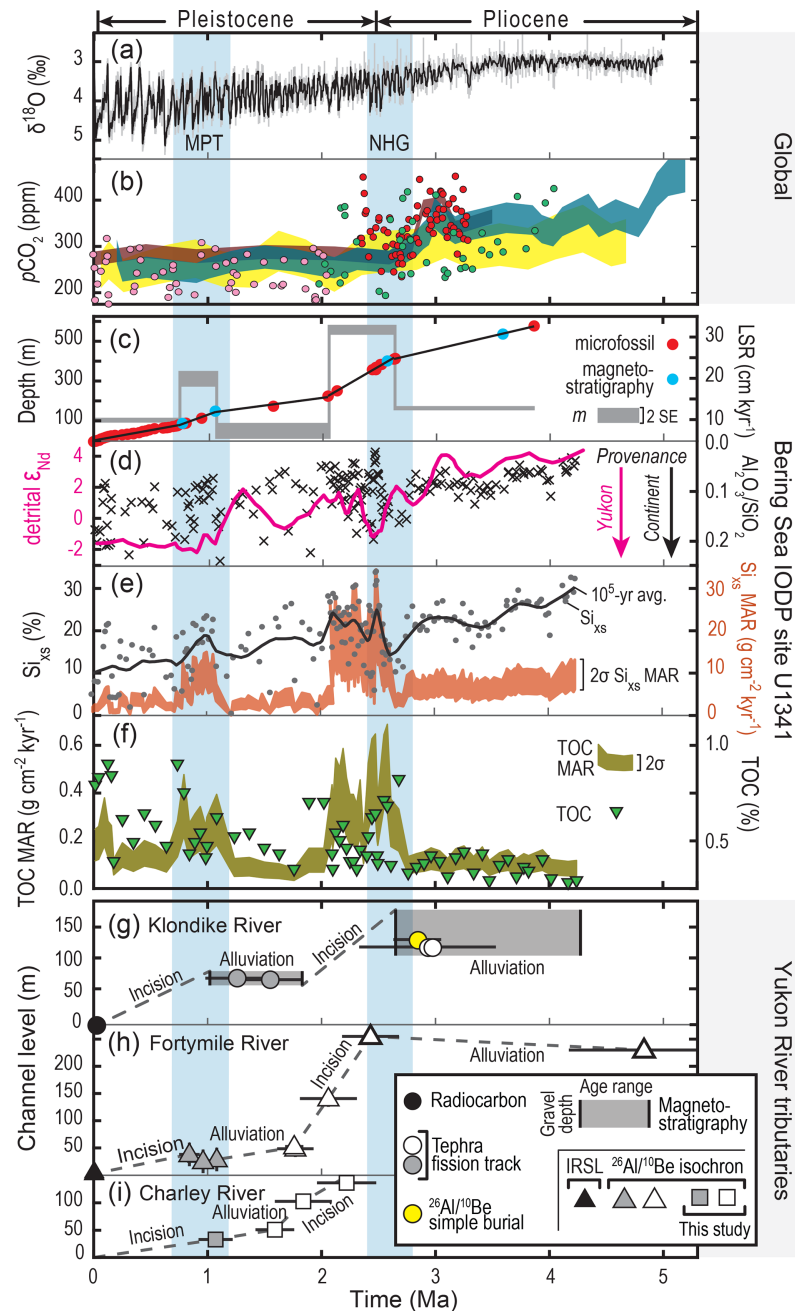
Figure 4. Late Cenozoic changes in global climate, Bering Sea sedimentation, and Yukon River tributary incision. (A) Global benthic \delta^{18}\text{O} (black line) and standard deviation (gray bars) (Ahn et al., 2017). (B) Atmospheric p\text{CO}_2 reconstructed from \delta^{11}\text{B} (red (Martínez-Botí et al., 2015), green (Bartoli et al., 2011), and pink (Hönisch et al., 2009) dots; blue envelope (Seki et al., 2010)) and alkenones (brown (Seki et al., 2010) and yellow (Pagani et al., 2010) envelopes). (C) Bering Sea integrated ocean drilling program (IODP) Site U1341 depth–age data (colored dots (Horikawa et al., 2015; Iwasaki et al., 2016)), regression model (black lines). Thick gray line plots regression model slope m and standard error (SE), which signify linear sedimentation rate (LSR) and uncertainty. (D) Detrital \text{Al}_2\text{O}_3/\text{SiO}_2 weight % ratio (black x's, higher ratios reflect more continental provenance (März et al., 2013)) and 10^5 yr moving average \epsilon_{\text{Nd}} values (magenta line, lower values reflect more Yukon River provenance (Horikawa et al., 2015)). (E) Silicate biomass inferred from weight % silica exceeding upper continental crust standard ( \text{Si}_{\text{xs}} ; gray dots (März et al., 2013)) and 10^5 yr moving average (black line), and \text{Si}_{\text{xs}} mass accumulation rate (MAR; orange envelope). (F) Total organic carbon (TOC; inverted triangles (März et al., 2013)) and TOC MAR (olive envelope). (G) Klondike River terrace ages over height above floodplain after composite magnetostratigraphy (Froese et al., 2000), tephrochronology (Westgate et al., 2003), cosmogenic burial dating (Hidy et al., 2013, 2018) and floodplain radiocarbon ages (Lowey, 2006). (H) Fortymile River terrace ages over height above the Middle to Late Holocene-aged floodplain (Bender et al., 2020). (I) Charley River terrace ages over height above the modern channel. MPT – Middle Pleistocene climate transition; NHG – Northern Hemisphere glaciation intensification.
