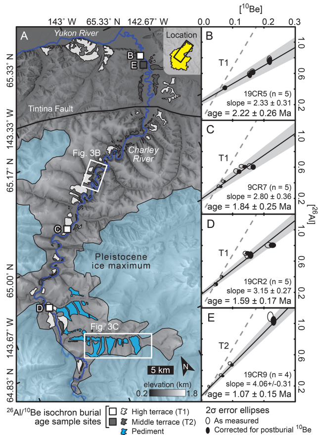
Figure 2. Charley River field area and cosmogenic results. (A) Charley River geomorphic map, terrace cosmogenic ^{26}\text{Al}/^{10}\text{Be} isochron burial age sample sites, and Pleistocene ice maximum (Kaufman et al., 2011; Duk-Rodkin et al., 2001) rendered on the IfSAR Alaska digital elevation model ( https://earthexplorer.usgs.gov/ , last access: 24 October 2022). White outlined boxes indicate areas photographed in Fig. 3b and c. (B–E) Cosmogenic ^{26}\text{Al}/^{10}\text{Be} isochron burial age plots for high (T1) and intermediate terraces (T2), isotope concentrations are in units of 10^6 \text{ atoms g}^{-1} quartz. Gray dashed line is the ^{26}\text{Al}/^{10}\text{Be} surface production ratio and \sim zero age, gray envelope is the 1σ regression uncertainty.
