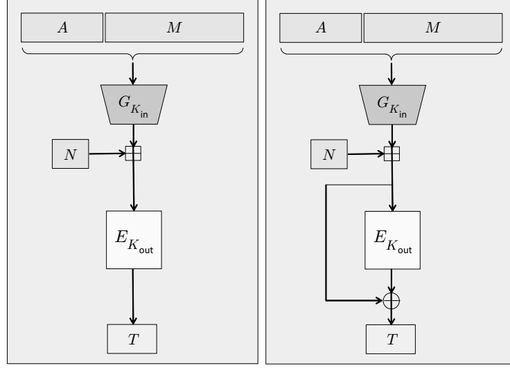
Fig. 11. The \text{GMAC}^+ construction (left) and its variant \text{GMAC2} (right).
