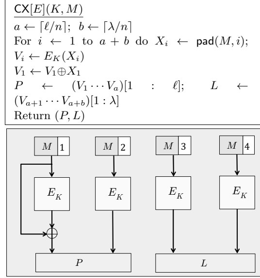
Fig. 13. The committing PRF scheme \mathbf{CX}[E, \text{pad}] , illustrated for the case \ell = \lambda = 2n and \text{pad}(M, i) is the concatenation of M and an (n - m) -bit encoding of i .
