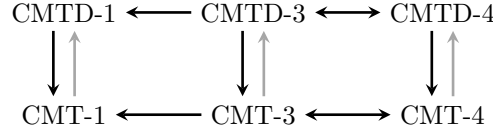
Fig. 4. Games defining committing security of a symmetric encryption scheme \text{SE} . Below them are the associated what-is-committed functions \text{WiC}_\ell , and then the relations between the notions. The gray arrows hold for tidy \text{SE} .
