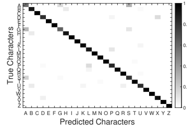
Fig. 15. Confusion Matrix of classification.
