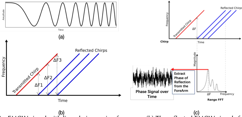
Fig. 5. (a) An FMCW signal with linearly increasing frequency (b) The reflected FMCW signals from objects in the environment (c) A range-FFT will result in multiple peaks corresponding to objects in the environment. Tracking the phase of the peak from forearm reflections will facilitate finger motion tracking
