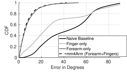
Fig. 7. The reflection from fingers ( Fingers-only ) do not capture sufficient reflections and the accuracy is close to naively predicting an always open palm. On the other hand, forearm reflections ( Forearm-only ) can provide reliable prediction of 3D finger motion. Accordingly, ForeArm reflections mainly contribute to the high accuracy in mm4Arm .
