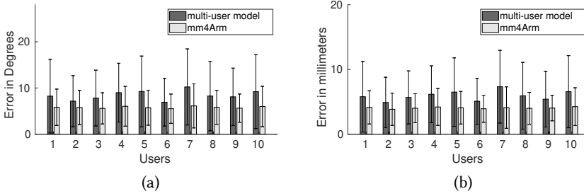
Fig. 13. mm4Arm with domain adaptation outperforms multi-user model for all users: (a) Error in degrees (b) Error in millimeters
