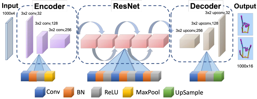
Fig. 10. Encoder Decoder Architecture. BN = Batch Normalization
