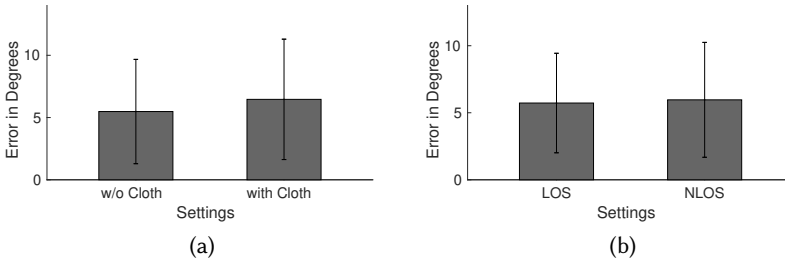
Fig. 14. (a) The accuracy remains stable when users wear long sleeve cloth (b) mm4Arm is robust to Non-Line-of-Sight conditions
