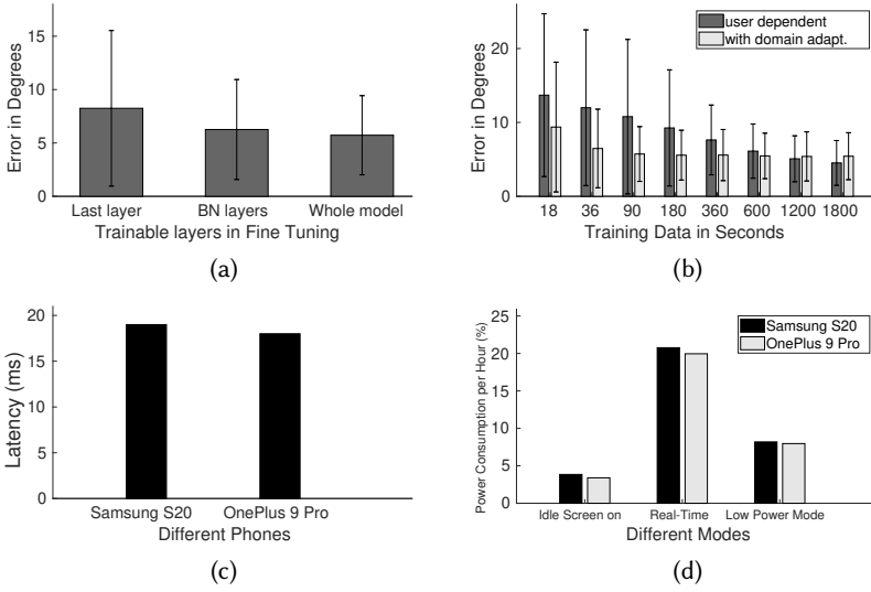
Fig. 19. (a) Accuracy comparison of different domain adaptation techniques. (b) Accuracy vs size of training data. (c) Latency of Execution and (d) Power Consumption on Smartphones
