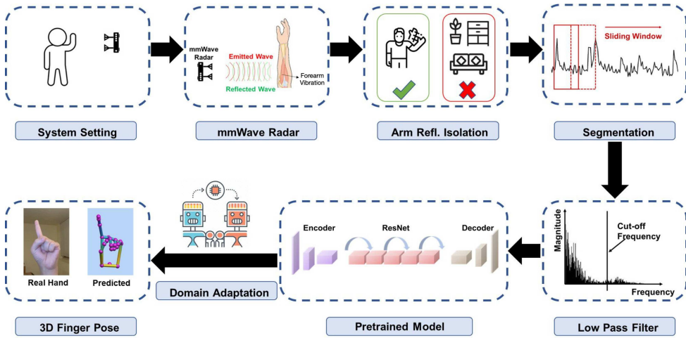
Fig. 1. mmWave reflections are captured from the surroundings from which the phases of arm reflections are first isolated. After subjecting the phase measurements to preprocessing techniques like low pass filters, deep learning based models are designed for extracting 3D finger motion from the phase data. Domain adaptation is incorporated in the design for decreasing the training overhead.
