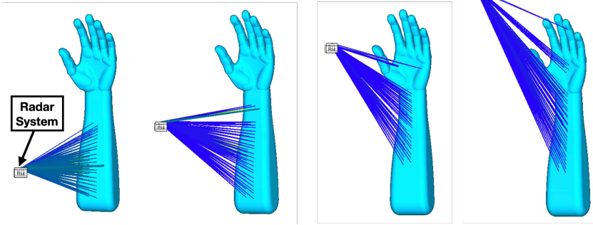
Fig. 6. Simulation results at 60 GHz: The blue lines visualize the rays that are transmitted and returning back to the radar via reflections. We vary the height of the radar to observe all surfaces on the hand that can yield stable reflections back to the radar. Results indicate that the reflections from fingers are negligible even when the radar is placed close to fingers. However, the large surface combined with texture and curvature of the forearm provides stable reflections for 3D finger motion tracking.
