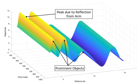
Fig. 8. Tracking of FMCW peaks over time helps eliminate noisy peaks. The phase data corresponding to the peak from the forearm reflection is used for 3D hand pose tracking
