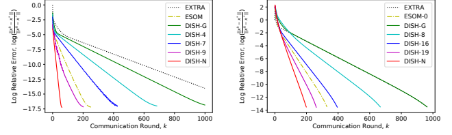
(a) Least Squares in Setup 1 (b) Logistic Regression in Setup 2 Fig. 3. Performance of EXTRA, ESOM-0, and DISH.
