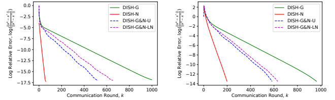
(a) Least Squares in Setup 1 (b) Logistic Regression in Setup 2 Fig. 4. Performance of DISH-G&N.
