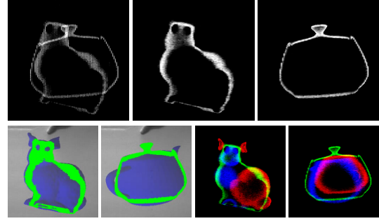
Figure 10. Our system can simultaneously capture multiple light curtains. Row 1: The demultiplexing process. In the leftmost raw image, even columns correspond to a bunny curtain while odd columns correspond to a teapot curtain. The separated curtains are shown in the middle and right images. Row 2: Sweeping a foam board through the curtains. Three positions of the board are represented by different colors in the two rightmost images.
