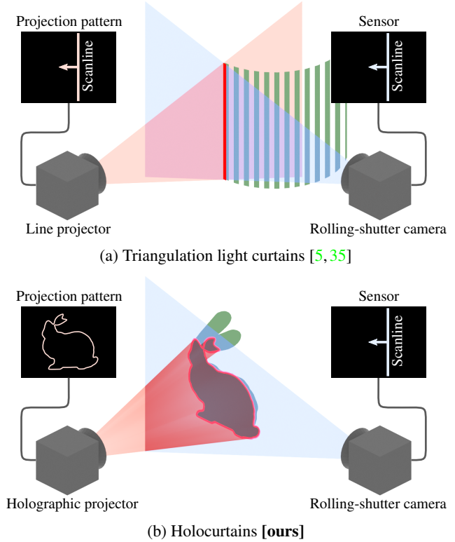
Figure 2. Illustration of light curtain systems. (a) A triangulation light curtain combines a laser line with either a 1D line sensor [35] or a rolling-shutter camera [5]. The light curtain (green) is formed at the intersection of the illumination plane (red) and sensing plane (blue), which are synchronously scanned together to form a ruled surface. (b) We propose using holographic projector that steers light to select regions of the scene at high speeds. The light curtain of a bunny is formed by synchronizing projection patterns (cross-sections of the bunny) with the rolling-shutter sensor.
