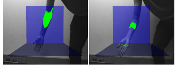
Figure 7. Our system can simultaneously form light curtains of different orientations. In this figure, we simultaneously place both a vertical and horizontal light curtain into the scene. Over the course of a single rolling-shutter exposure, our system is able to detect objects intersecting either of these curtains.
