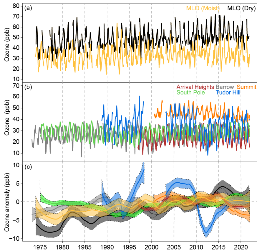
Fig. 2.64. (a) Nighttime monthly mean ozone values (ppb) at Mauna Loa (MLO), split into mutually exclusive times series, representing moist air (yellow, primarily a tropical origin) and dry air (black, primarily a midlatitude origin) based on observed relative humidity values (Gaudel et al. 2018). (b) Monthly mean surface ozone (ppb) at Barrow Observatory, Alaska (gray), Summit, Greenland (orange), Tudor Hill, Bermuda (blue), Arrival Heights, Antarctica (red), and South Pole (green). Monthly means are produced for months with at least 50% data availability, using observations from all 24 hours of the day. The locations of each site are listed in Table 2.11. (c) The same time series after conversion to monthly anomalies referenced to the monthly climatological values over 2000–20 and smoothed variability based on the LOWESS (locally weighted scatterplot smoothing) regression.
