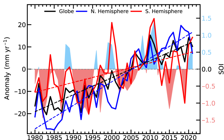
Fig. 2.38. Land evaporation anomaly ( \text{mm yr}^{-1} ; 1991–2020 base period) for the NH, SH, and the entire globe (blue, red, and black solid lines, respectively). Linear trends in evaporation (dashed lines) and the Southern Oscillation Index (SOI) from CRU (right axis, shaded area) are also shown. (Source: GLEAM.)
