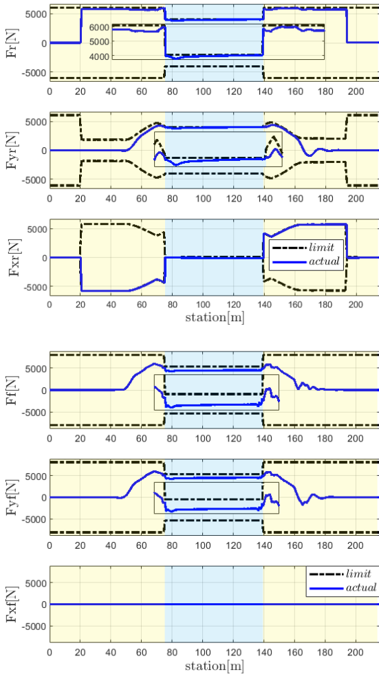
Figure 9. Tire forces: (a) rear tire; (b) front tire.
