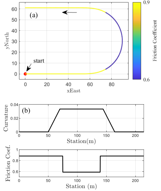
Figure 1. Sample path: (a) path shape; (b) path curvature and friction coefficient.
