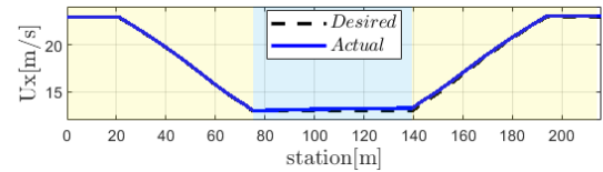
Figure 6. Vehicle speed.
