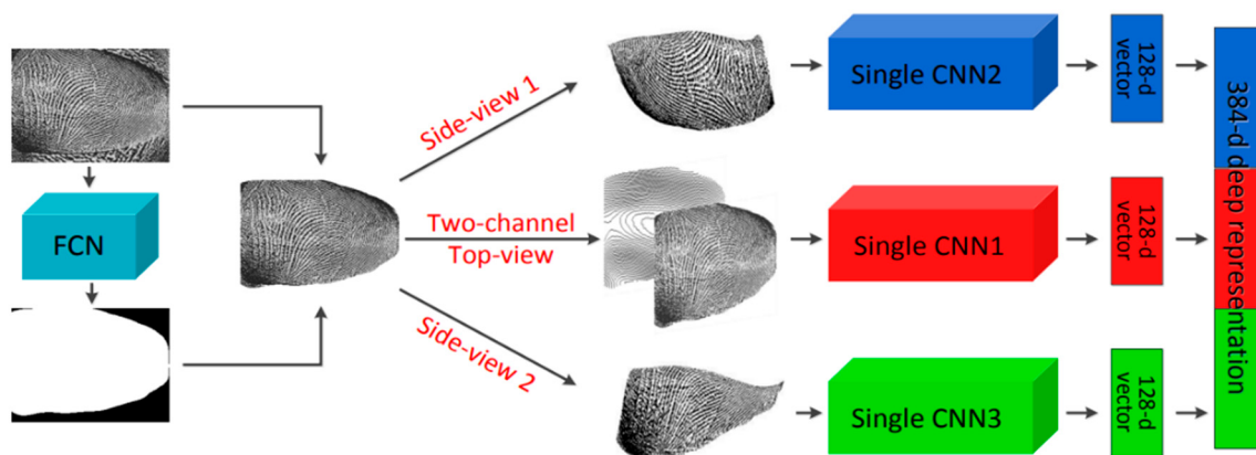
Figure 11. Automatic learning of 3D fingerprint features via deep representation [86].
