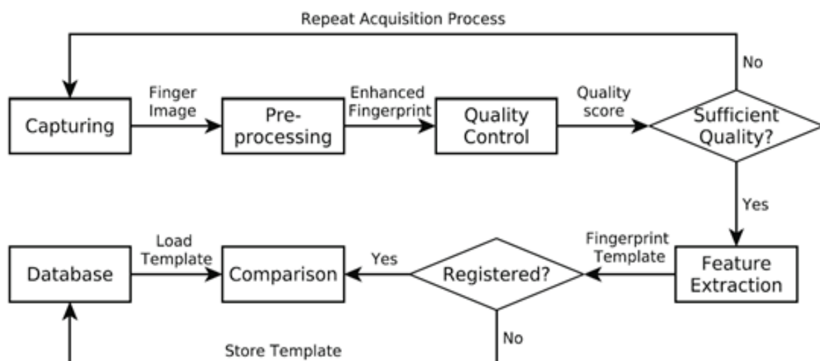
Figure 3. Overview of the sub-systems of a generic contactless fingerprint recognition system [10].
