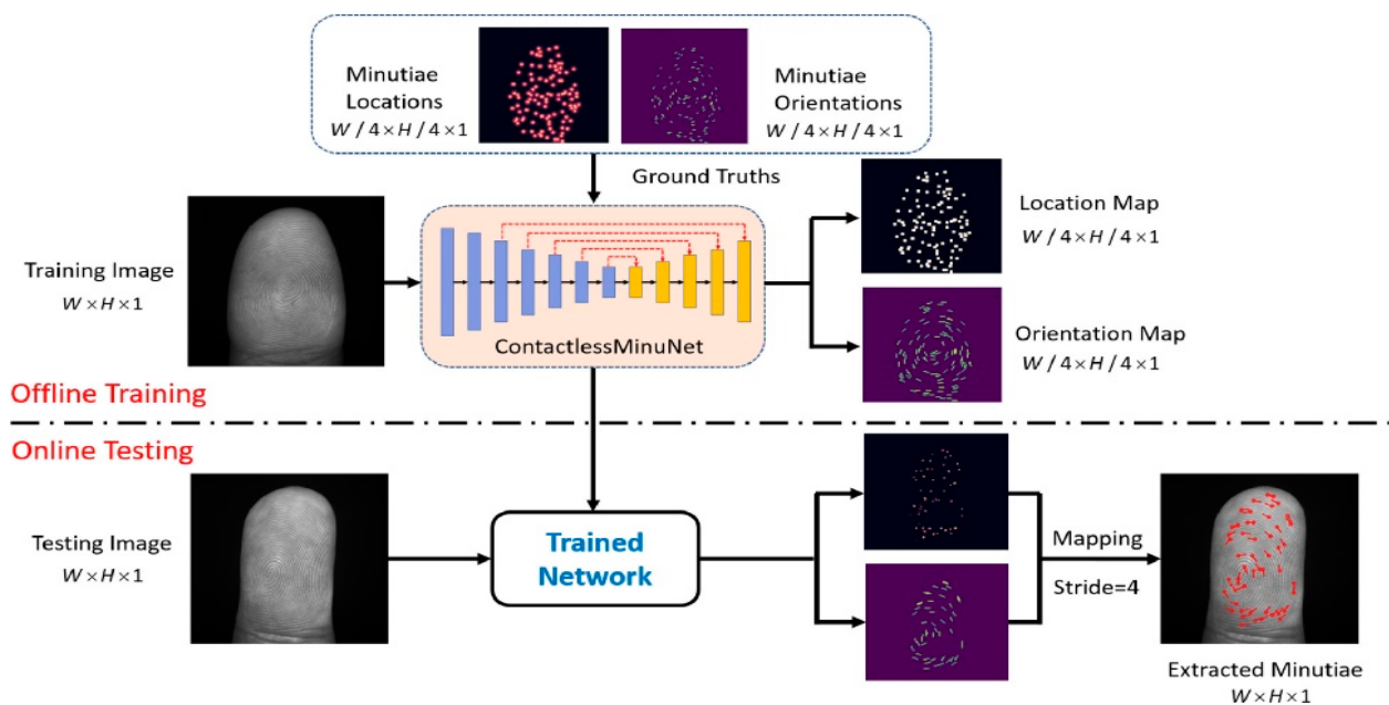
Figure 9. Overview of the minutiae extraction algorithm for contactless fingerprints based on multi-task fully deep convolutional neural network [2].
