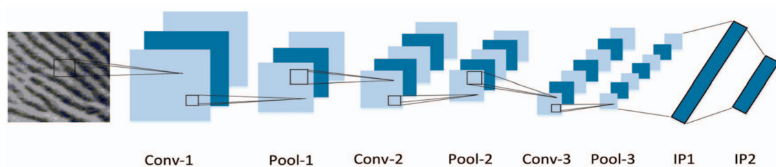
Figure 10. JudgeNet and LocalNet share a similar convolutional architecture [82].
