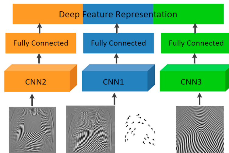
Figure 12. Deep-feature representation generation process using three multi-Siamese networks [83].
