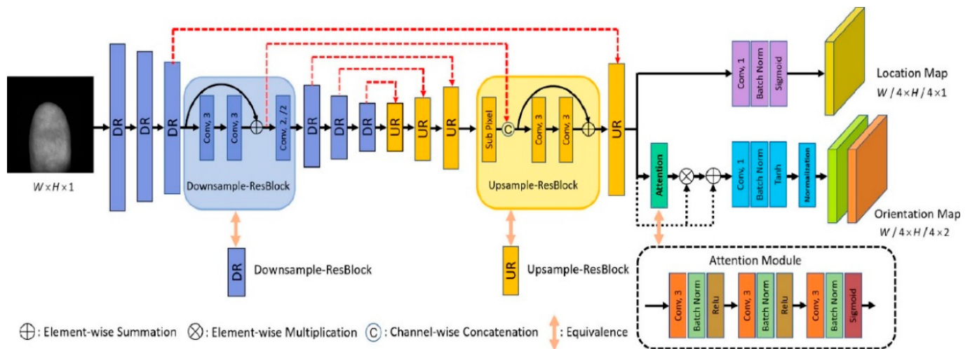
Figure 8. An architecture of multi-task deep convolutional networks [79].
