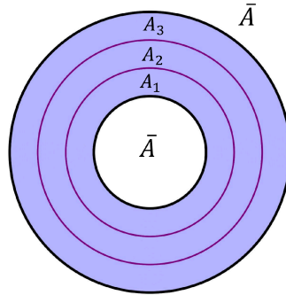
Figure 5: In the above figure we set A = A_1 \cup A_2 \cup A_3 to be an annulus whose inner and outer radius is R_1 and R_2 . It is divided into three smaller annuli by the two purple circles.
