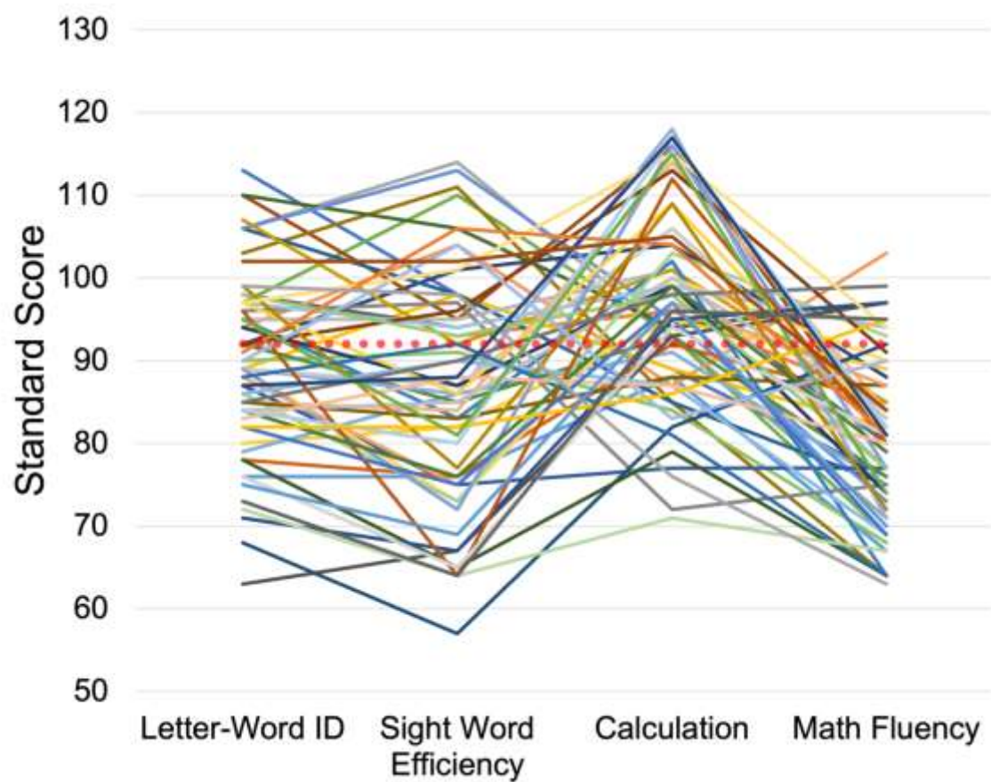
Figure 1. Reading and Math standard scores for each of the 63 children. The dotted red line represents a standard score of 92.
